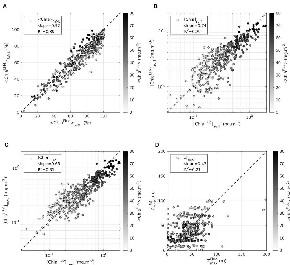
FIGURE 5 Assessment of the LFM performance on the validation sample. Values in the horizontal axis are metrics derived from the observations ( [Chla^{Fluo}] ). Values in the vertical axis are metrics derived from the predictions ( [Chla^{LFM}] ). The metrics examined to assess the performance of the LFM are (A) [Chla^{Fluo}]_{\%ML} , the percentage of Chla in the mixed layer (B) the surface value of [Chla], [Chla^{Fluo}]_{surf} (C) the maximum value of [Chla], [Chla^{Fluo}]_{max} and (D) Z_{max}^{Fluo} , the depth of the maximum value of [Chla]. The dashed black lines in each plot represent the 1:1 reference line. The metrics ( R^2 , slope) associated with the linear regression performed between model predictions and observations are indicated in each plot.
