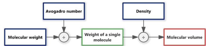
Fig. 7. Schematic of molecular volume calculations.
