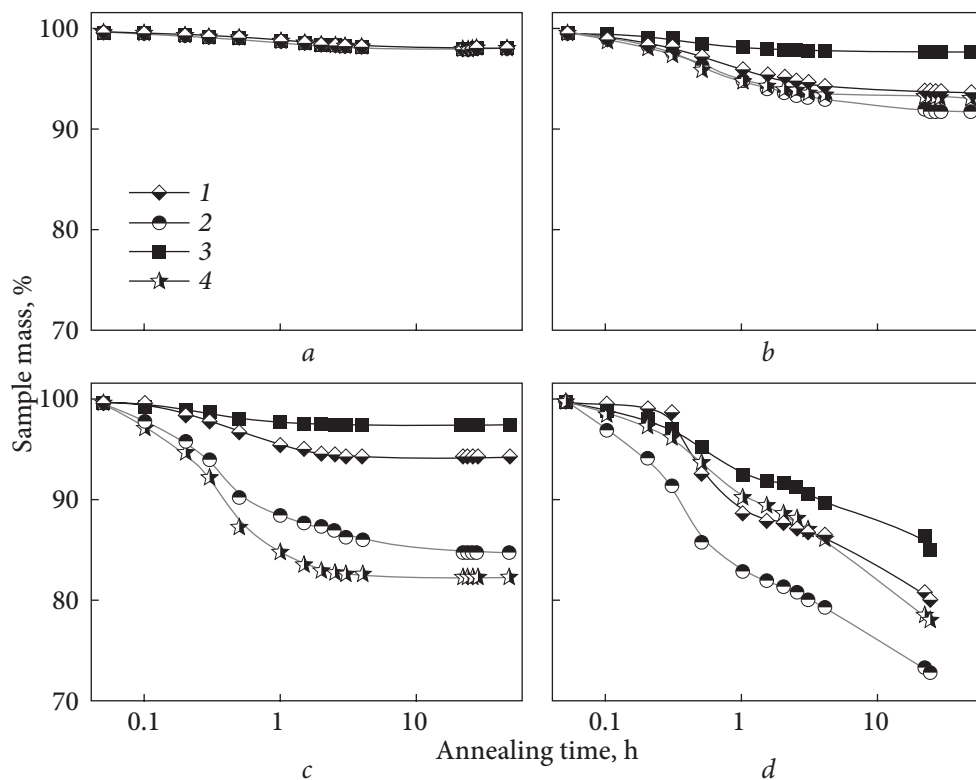
Fig. 3.12. Isothermal thermogravimetric curves for nanoporous samples: PCN DOP20 (1), PCN DBP30 (2), PCN DMP30 (3), and PCN DMP50 (4). Annealing was performed at T_a equal to 50 °C (a), 100 °C (b), and 150 °C (c) for 48 h or 250 °C for 24 h (d)
