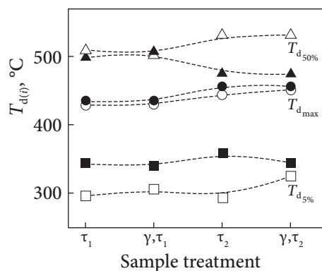
Fig. 6.7. Temperatures of thermal degradation ( T_{d(i)} ) versus sample treatment method for nanoporous grafted semi-IPNs: CER-A/LPU (solid symbols) and CER-E/LPU (open symbols). The T_{d5\%} , T_{d50\%} , and T_{dmax} are the temperatures corresponding to the indicated sample mass losses (subscript) and maxima of DTG peaks, respectively
