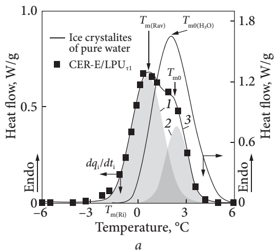
Fig. 6.3. Typical (a) DSC thermoporometry curves for melting ice crystallites of pure water and ice crystallites of water inside the swollen nanoporous CER-E/LPU _{\tau 1} sample (indicated in the plot); curves 1, 2, and 3 correspond to the Gaussian fitting of the thermoporometry multi-peak curve for the CER-E/LPU _{\tau 1} sample: 1 — for melting ice crystallites inside pores, 2 — for melting ice crystallites in the bulk sample, and 3 — cumulative curve of the approximation; b, c — Pore size distribution curves by DSC thermoporometry for different nanoporous CER-E/LPU grafted semi-IPNs (indicated in the plots)
