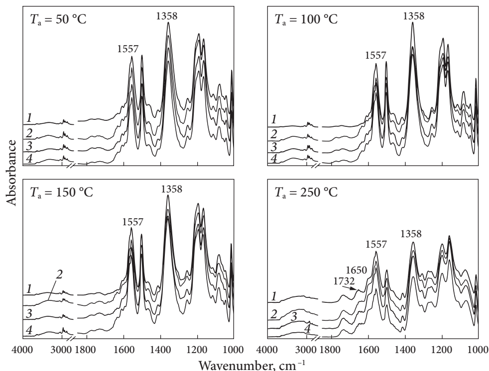
Fig. 3.14. FTIR spectra of nanoporous samples after annealing at different temperatures for PCN DOP20 (1), PCN DBP30 (2), PCN DMP30 (3), and PCN DMP50 (4). The curves are shifted vertically for the sake of clarity
