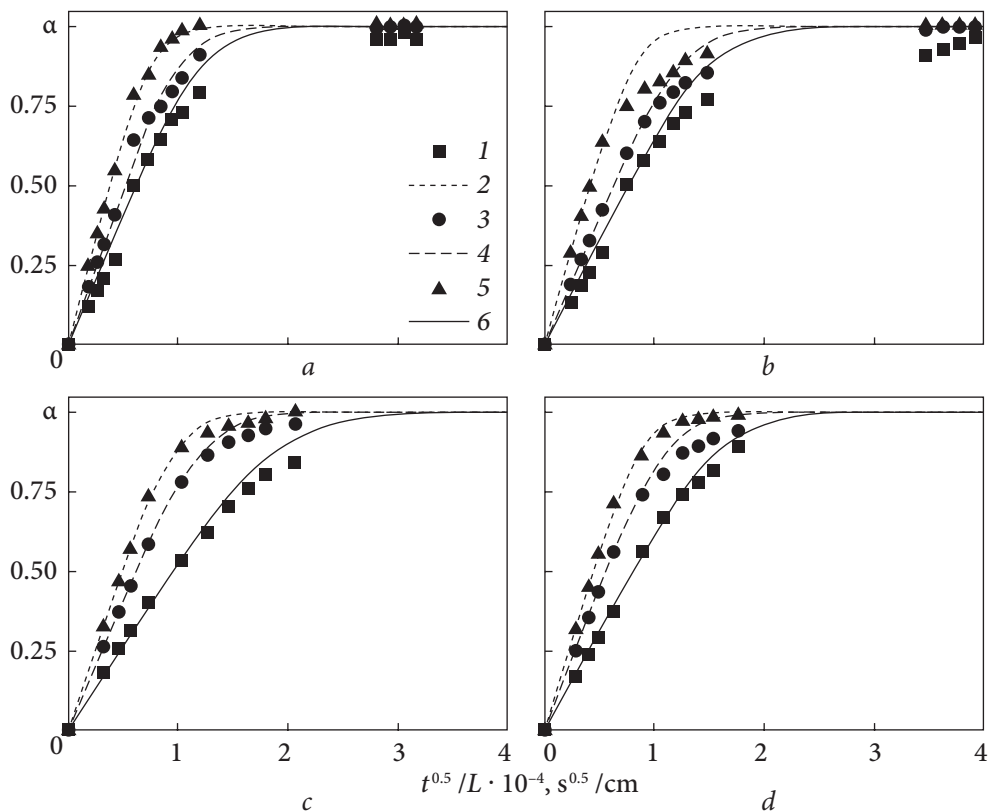
Fig. 3.15. Dependence of conversion ( \alpha ) on t^{0.5}/L for nanoporous PCN_{DOP20} (a), PCN_{DBP30} (b), PCN_{DMP30} (c), and PCN_{DMP50} (d) samples during annealing. Symbols represent the experimental data and dashed curves correspond to the theoretical values (as determined by Eqs. 3.1 and 3.2). Annealing was performed at 50 °C (1, 2), 100 °C (3, 4), and 150 °C (5, 6)
