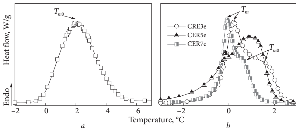
Fig. 5.5. Typical DSC melting thermograms of (a) bulk deionized water and (b) water confined within the pores of different nan porous CER structures investigated
