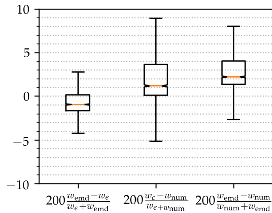
Figure 7. Comparison of the different ways to compute the Wasserstein distance over the realistic database. Relative errors in percent between w_{\text{emd}} , w_{\text{num}} , and w_\epsilon . The orange line is the median. Box boundaries are defined by the first and the third quartiles. The whiskers are set at 150 % of the inter-quartile range.
