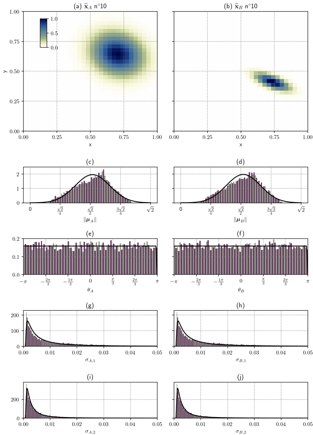
Figure 4. Characteristics of the Gaussian puff database. (a, b) Images A (a) and B (b) number 10. (c–j) Histograms of \|\mu_A\| (c) , \|\mu_B\| (d) , \theta_A (e) , \theta_B (f) , \sigma_{A,1} (g) , \sigma_{B,1} (h) , \sigma_{A,2} (i) , and \sigma_{B,2} (j) .
