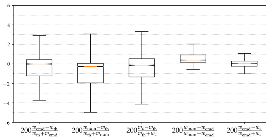
Figure 5. Comparison of the different ways to compute the Wasserstein distance over the Gaussian puff database. Relative errors in percent between w_{\text{emd}} , w_{\text{th}} , w_{\text{num}} , and w_{\text{e}} . The orange line is the median. Box boundaries are defined by the first and the third quartiles. The whiskers are set at 150 % of the inter-quartile range.
