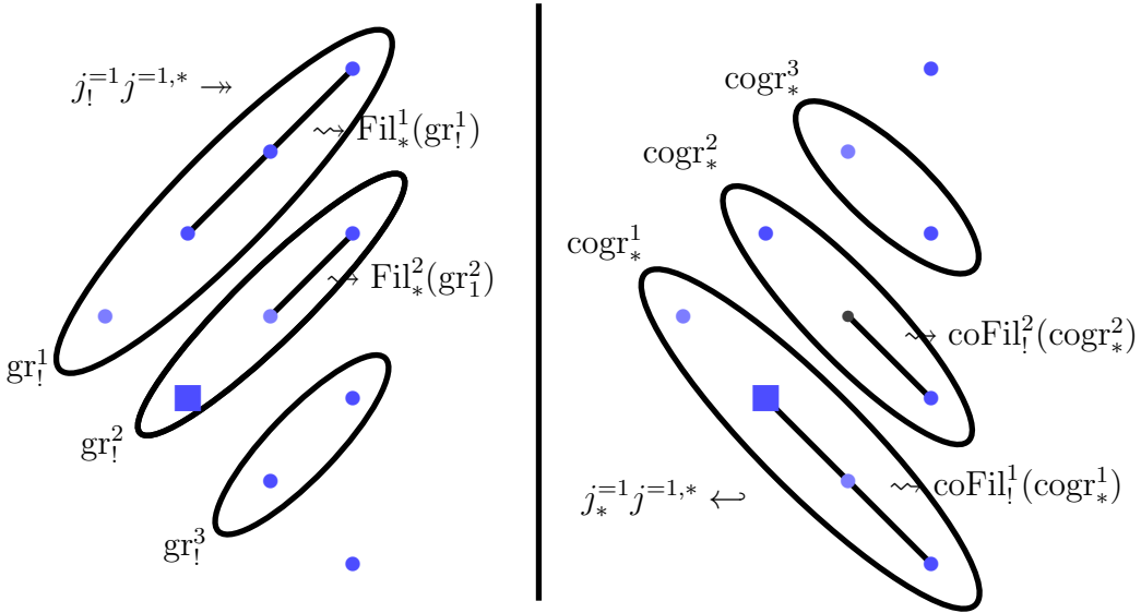
FIGURE 1. Filtrations of stratification of \Psi_{K,\varrho} for \varrho a character
