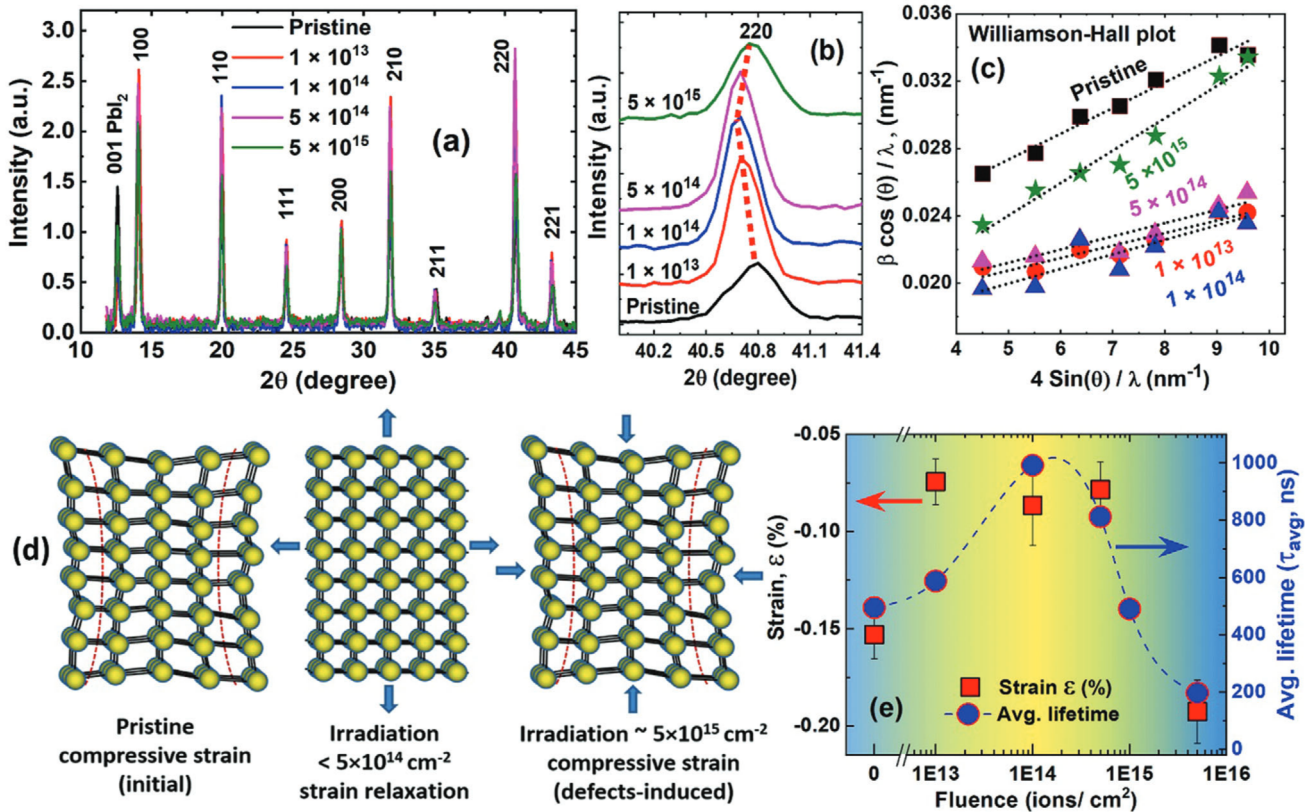
Figure 2. a) X-ray diffraction (XRD) spectra of triple-cation mixed-halide perovskite films at different irradiation fluences. b) (220) diffraction peak, the red dotted line illustrates the complex strain behavior as a function of irradiation fluences. c) Linear Williamson Hall plot of the XRD data for pristine and irradiated films at different fluences. d) Schematic for ion irradiation and strain modification on an MHP sample. e) Correlation between average carrier lifetime and compressive strain as a function of irradiation fluence (relative strain is estimated from WH analysis of the XRD measurements, and average lifetime is estimated from the TCSPC data).
