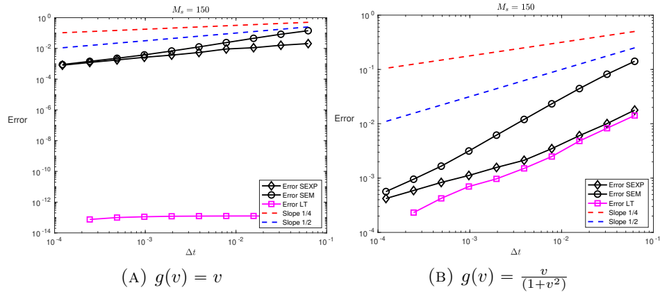
FIGURE 3. SPDE in 2d : Mean-square errors of the splitting scheme (LT), the stochastic exponential Euler integrator (SEXP), and the semi-implicit Euler–Maruyama scheme (SEM). Mesh sizes h_{x_1} = h_{x_2} = 2^{-4} and average over 150 samples.
