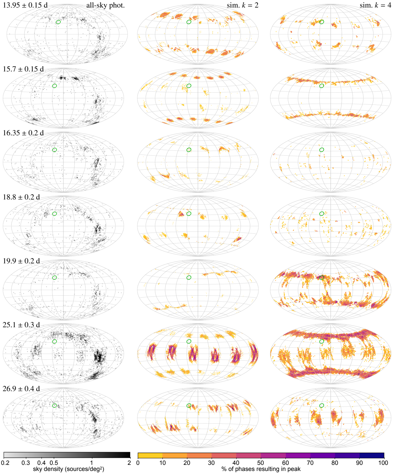
Fig. C.2. Ecliptic Aitoff projection of the photometric data presented in Fig. 22. Left: Source density of the photometric peaks for the all-sky sample (top panel of Fig. 22). Right: Result of the all-sky uniform simulations of our noiseless sampled bias model (panels 2 and 3 of Fig. 22). They are colour-coded with the percentage of phases (position angles) that results in this peak: A low value means that only specific phasing of the scan-angle signal will result in a particular peak being observed at the given location. The green circle indicates the location of the GAPS catalogue (see Fig. 23). In all sky plots, longitude zero is at the centre and increasing to the left.
