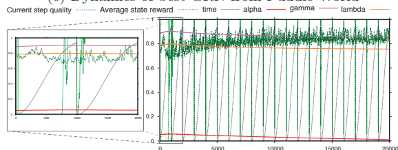
(g) Dynamics of best GRN from Acrobat
