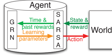
Figure 1: At every time step, SARSA updates the GRN inputs. The GRN returns updated learning parameters that are used by the SARSA algorithm.
