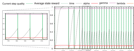
(a) Dynamics of best GRN from Mountain Car
