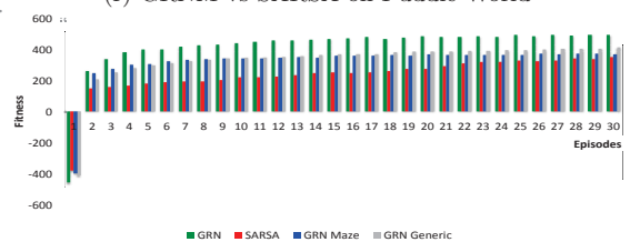
(h) GRNM vs SARSA on Acrobat
