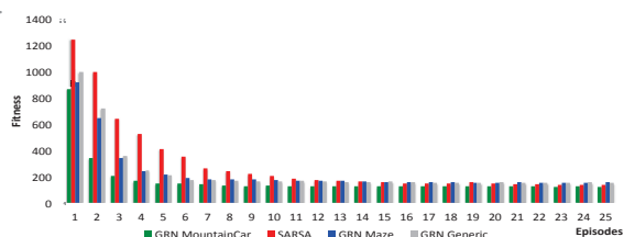
(b) GRNM vs SARSA on Mountain Car
