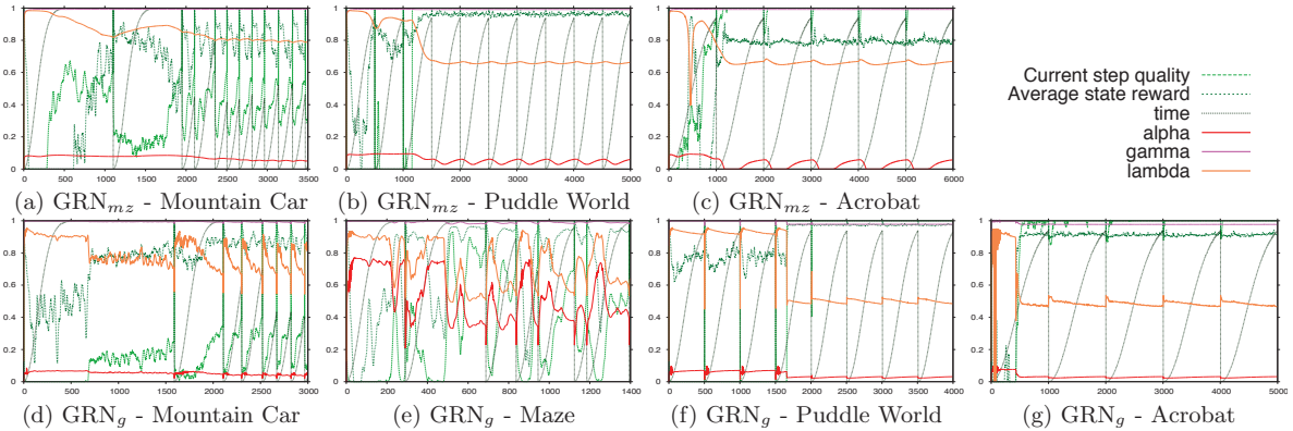
Figure 4: (a-c) Behavior of the GRN trained on the Maze problem when used on other problems; (d-g) Behavior of the generic GRN when used on all problems.
