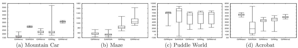
Figure 5: Detailed results of the 100 runs from the four problems with the best GRN trained on the specific problem, the SARSA algorithm with fixed parameters, the GRN trained on Maze (noted GRN_{mz} in the box plots), and a generic GRN trained both on the Maze and Mountain Car problems (noted GRN_g ). Notice that, for the first two problems (Mountain Car and Maze), lower is better and for the two others (Puddle World and Acrobat), higher is better.
