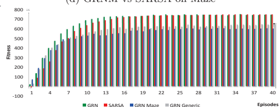
(f) GRNM vs SARSA on Puddle World
