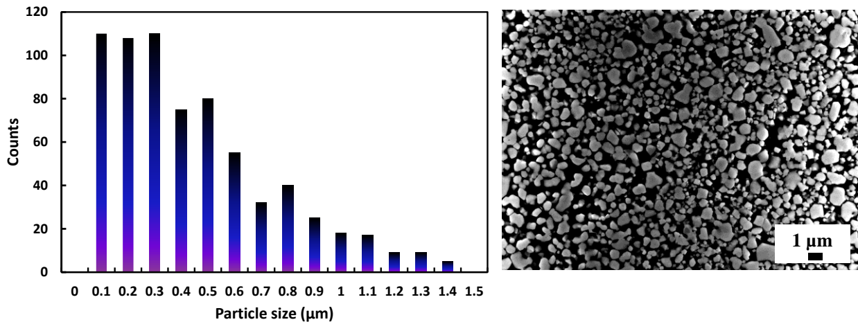
Figure A Histogram of initial powder grain size distribution and SEM image of initial grains.
