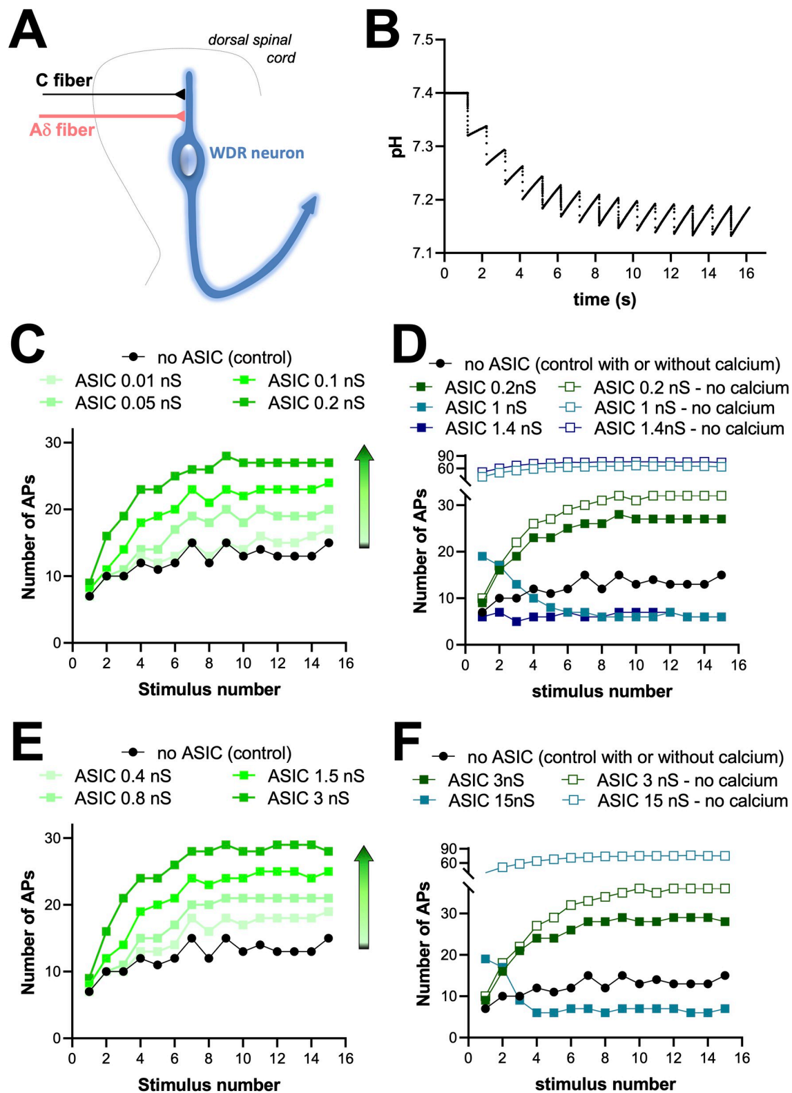
Fig 4. Computational model of WDR neuron with ASIC1a channel parameters and a synaptic cleft acidification system. A , Schematic representation of the computational model used, with a WDR projection neuron receiving directly a 20-synapse connection from both A \delta -fibers and C-fibers. B , Simulation curve showing the evolution of synaptic pH as a function of time during windup-inducing stimulations. C , Simulation windup curves obtained without (control, no ASIC, black dots) and with moderate
