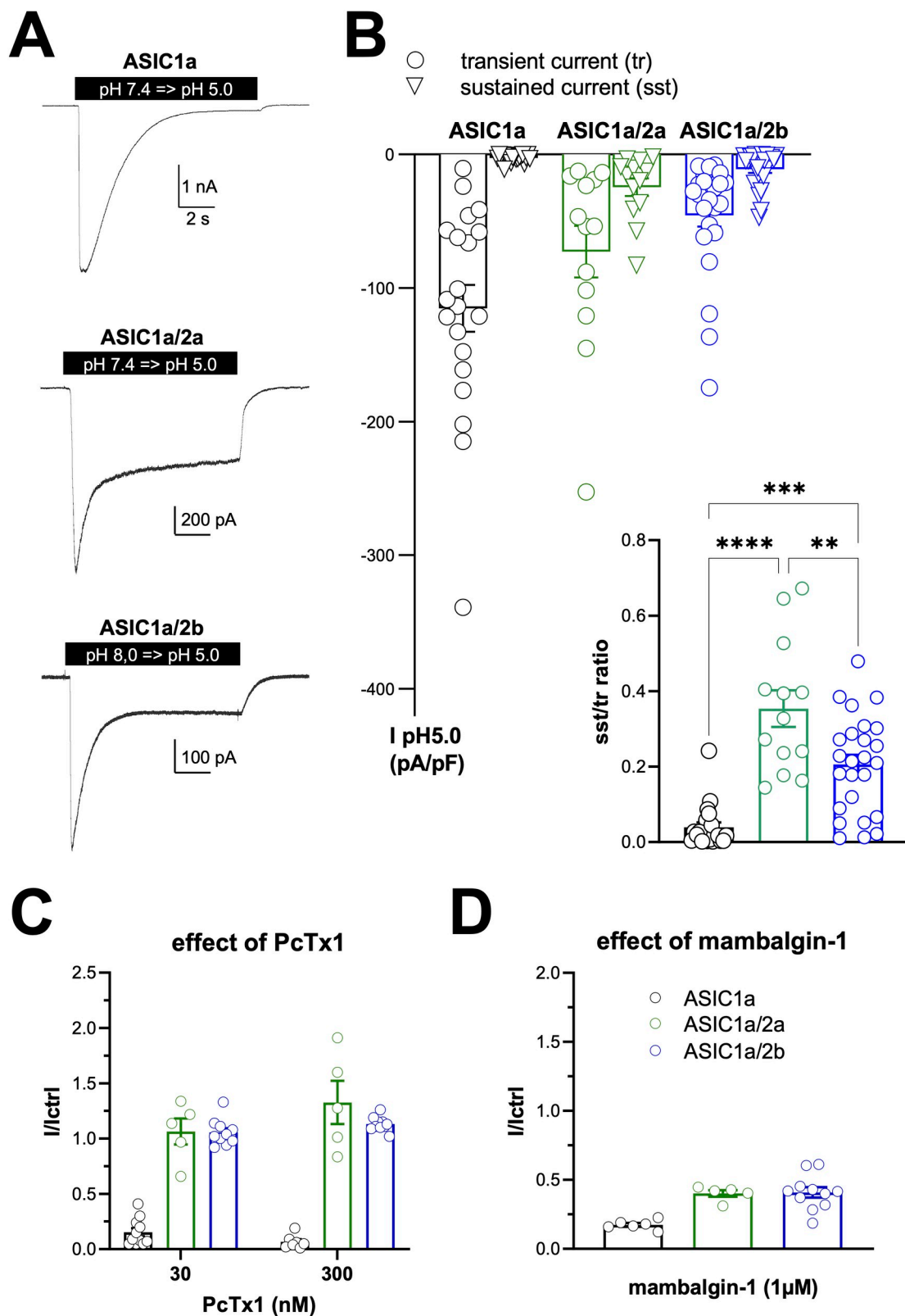
Fig 3. Effects of PcTx1 and mambalgin-1 on ASIC1a homomeric and heteromeric channels. A, Typical ASIC1a, ASIC1a/2a and ASIC1a/2b currents recorded at -50 mV from HEK293 transfected cells following extracellular acidification to pH5.0. B, Statistical analysis of the current densities recorded in A. Both the transient (tr) and sustained (sst) currents were measured, and the ratio sst/
