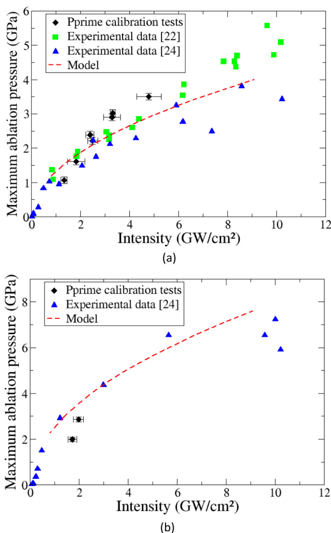
FIG. 7. Maximum ablation pressure measurements as a function of intensity for water confinement and comparison with the analytical model (with \alpha = 0.2 ) (a); for glass confinement and comparison with the analytical model (with \alpha = 0.15 ) (b).
