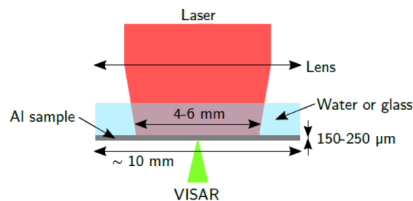
FIG. 5. Laser-driven shock tests performed at the Institut Pprime on aluminum. The free surface velocity was monitored with a VISAR represented by the green beam.
