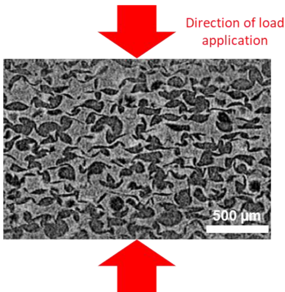
FIG. 13. In situ tomograph of a foam sample subjected to a quasi-static compression.
