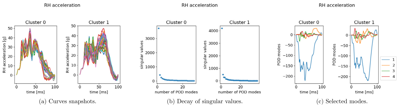
Fig. 26. POD results for RH x-acceleration snapshots within the two identified clusters.
