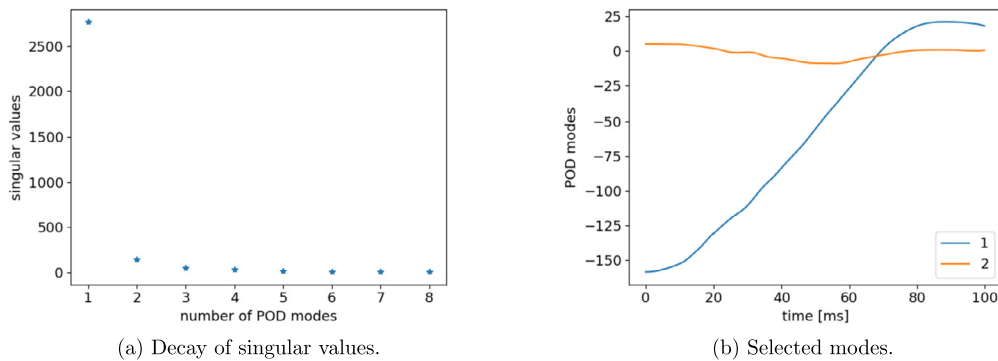
Fig. 9. POD results for LH x-velocity snapshots.
