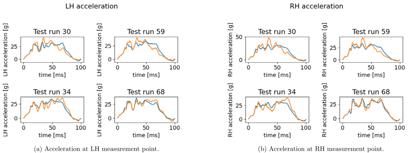
Fig. 19. Reconstructed x -acceleration using the sPGD models (orange: Hi-Fi simulation, blue: Reduced Model).
