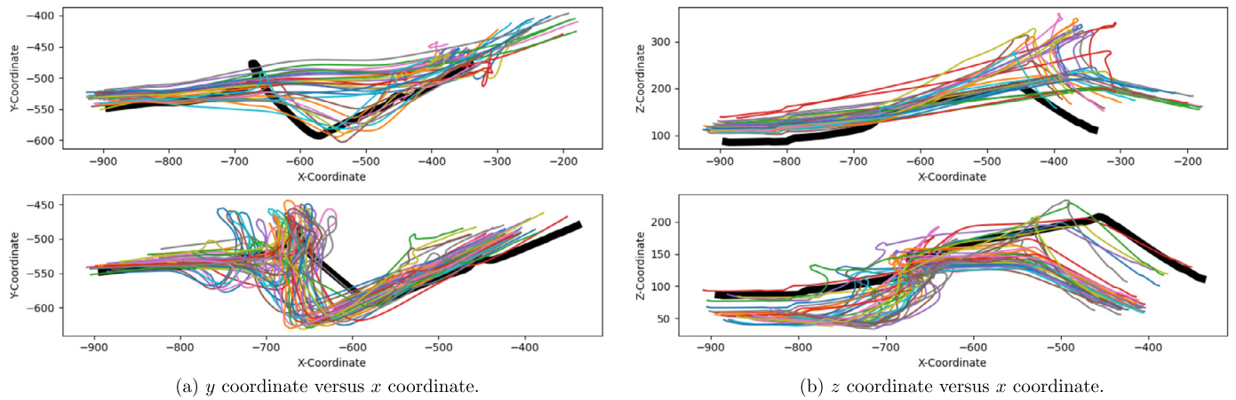
Fig. 24. Two clustered deformation modes (up and down); black fat line representing the reference mode.
