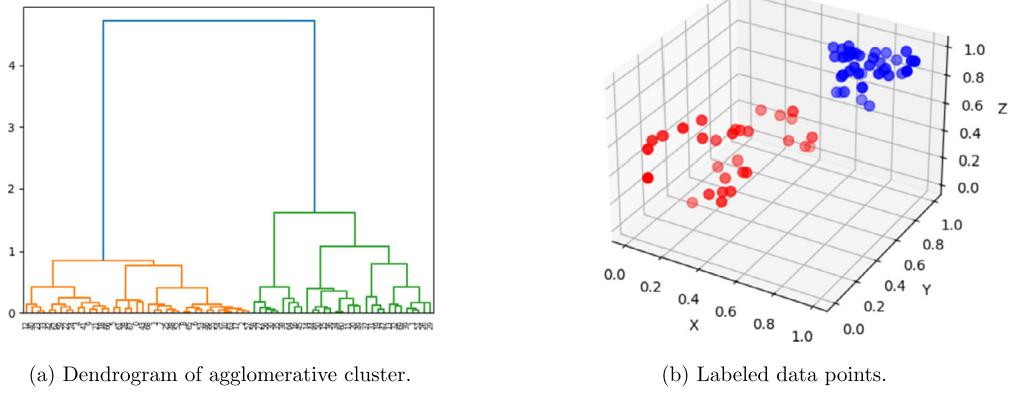
Fig. 23. Hierarchical clustering results.
