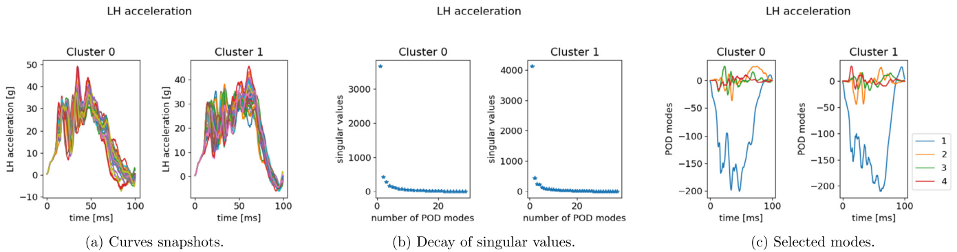
Fig. 25. POD results for LH x-acceleration snapshots within the two identified clusters.
