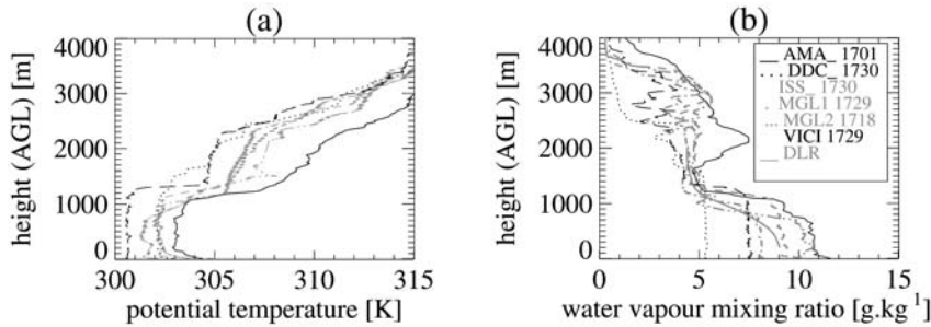
Figure 3. Vertical profiles from soundings on 14 June 2002 around 1700 UTC: (a) potential temperature (K) and (b) water-vapour mixing-ratio (g kg -1 ) (for which the light grey solid line denotes the mean DIAL lidar profile obtained from three segments centred over Homestead between 1700 and 1730 UTC). In both panels, other grey lines denote soundings launched in the sub-domain shown in Fig. 1(b).
