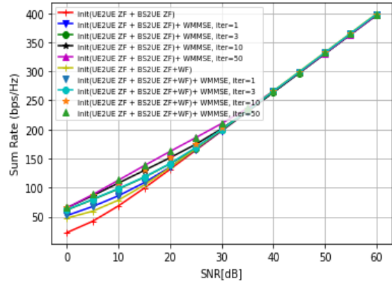
Fig. 4: sum rate performance with N_{ul} = 3, N_{dl} = 6, K_{ul} = 2, K_{dl} = 4 and r = 2
