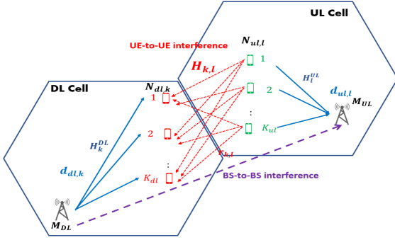
Fig. 1: DynTDD system Model
