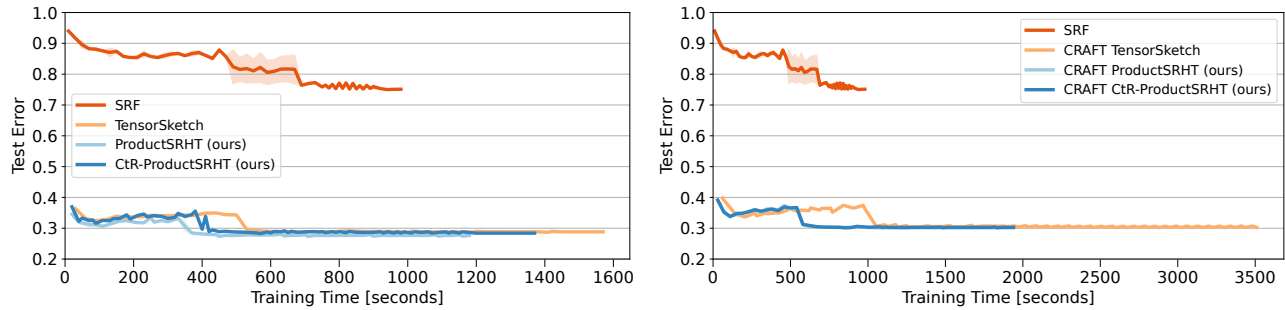
(a) (CtR-) ProductSRHT vs. TensorSketch/SRF.
