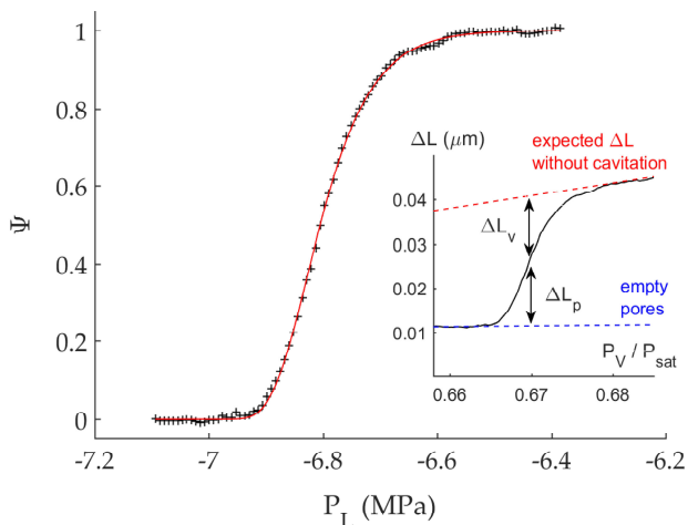
FIG. 5. Fraction \Psi of pores that have not cavitated at pressure P_L : experimental points (crosses) and fit by the double exponential of the equation 4 (red solid curve). Inset: close-up of the cavitation step of fig. 1. The dotted curves represent the signal \Delta L_0 for "empty" pores (blue) and the extrapolated signal (red) that would be observed without cavitation.
