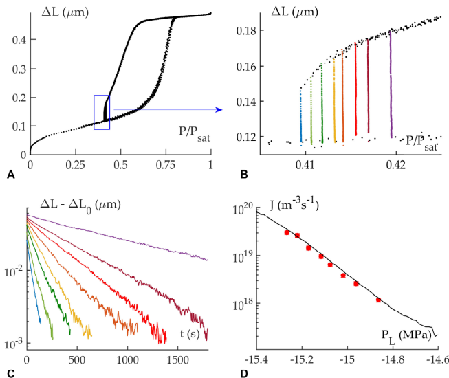
FIG. 4. (A) Optical isotherms measured in nitrogen at 73 K on the porous alumina sample C (see tab. I) during quenching at various pressures. The total measurement time is about 48 h. (B) Close-up of the isotherms showing the relaxations at constant pressures 239.7, 240.36, 241.07, 241.86, 242.41, 243.24, 244.04, 245.51 mbar. (C) Relaxation of \Delta L - \Delta L_0 at constant pressures (same values as in B). \Delta L_0 stands for the optical thickness of empty pores ( \Delta L_0 \simeq 0.12 \mu\text{m} , a small variation is allowed from run to run to account for the small long term drift). (D) Nucleation rate J as a function of the relaxation time measured in fig. C (squares - the size of the symbols sets the uncertainty) and from the shape of the isotherm measured at constant pressure rate (line).
