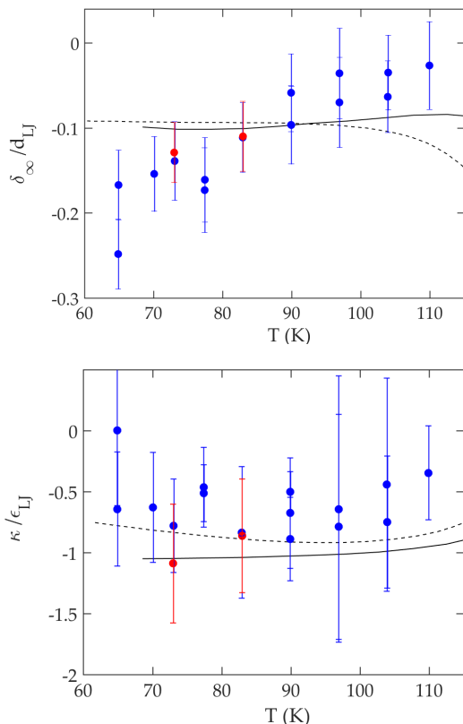
FIG. 7. Top : normalised asymptotic Tolman length \delta_\infty/d_{LJ} . Bottom: normalised rigidity constant \kappa/\epsilon_{LJ} . Lines are the results of DFT calculations: full line from ref. [11], dashed line from ref. [12].
