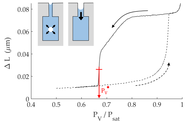
FIG. 1. Nitrogen optical isotherm at 90 K for the porous alumina sample A (mean pore diameter 33 nm, see table I). Upon decreasing the pressure, menisci start to recede in the larger apertures at P_V \simeq 0.8P_{\text{SAT}} , until cavitation occurs around 0.67P_{\text{SAT}} . Inset: sketch of meniscus receding (right) and cavitation (left) in an ink-bottle pore.
