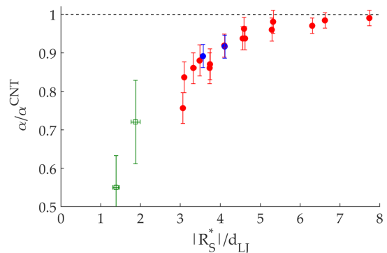
FIG. 6. Plot of \alpha = \frac{1}{k_B T} \left. \frac{\partial E_B}{\partial P_L} \right|_T , normalised by its CNT value calculated from eq. 1. Blue disks: this work, from the isotherm shape. Red: this work, from relaxation after quenching. Green open square are data for argon condensation, derived from the work of Sinha et al. [26]. Note that argon values for \alpha are plotted as a function of the critical EDS radius R_E since the stress radius R_S cannot be derived from [26].
