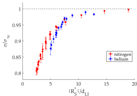
FIG. 3. Normalised surface tension as a function of the normalised bubble curvature |R_s^*|/d_{LJ} . Data for helium are measured above the superfluid transition. d_{LJ} for helium and nitrogen are given in the text. The temperature range is 65–120 K for nitrogen and 2.3–4.5 K for helium. The uncertainty on \sigma_\infty is about 1% and is not taken into account in the evaluation of the error bars (see Supporting Information).
