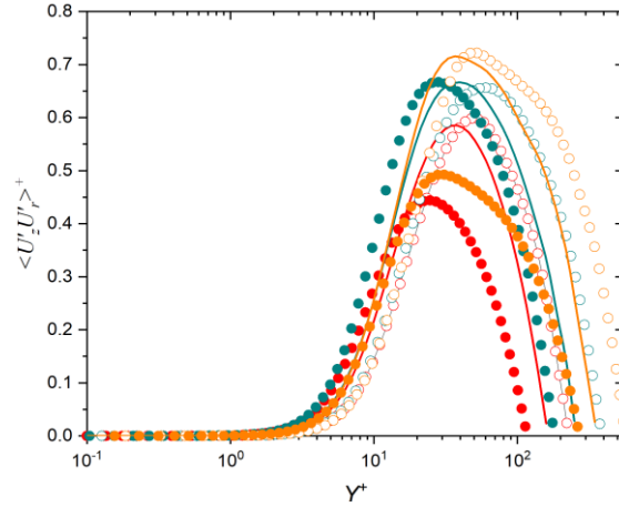
Figure 7: Turbulent Reynolds stress versus Y^+ .
