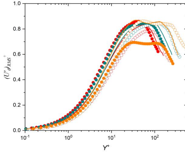
Figure 5: RMS of the tangential component versus Y^+ .
