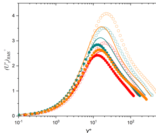
Figure 3: RMS of axial component versus Y^+ .
