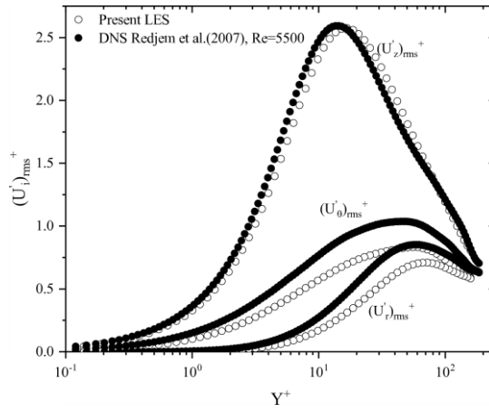
Figure 2: Validation of the results.
