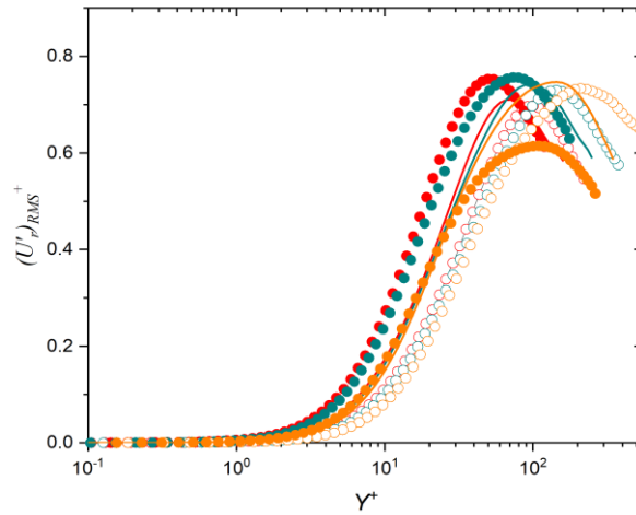
Figure 4: RMS of the radial component against Y^+ .
