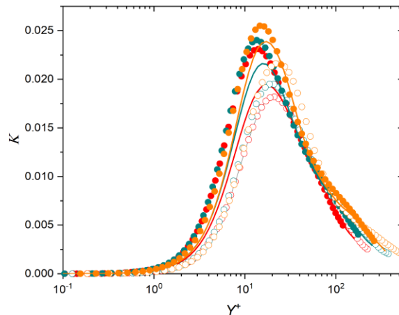
Figure 6: Turbulent kinetic energy against Y^+ .
