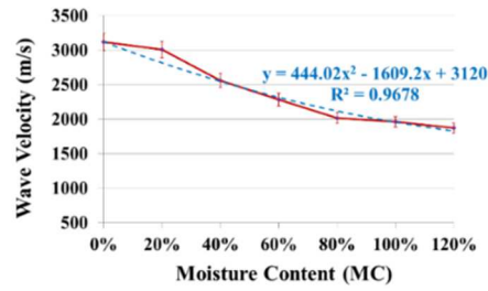
Fig. 5. Correlations between AE wave velocity and MC of GFRP-balsa sandwich.
