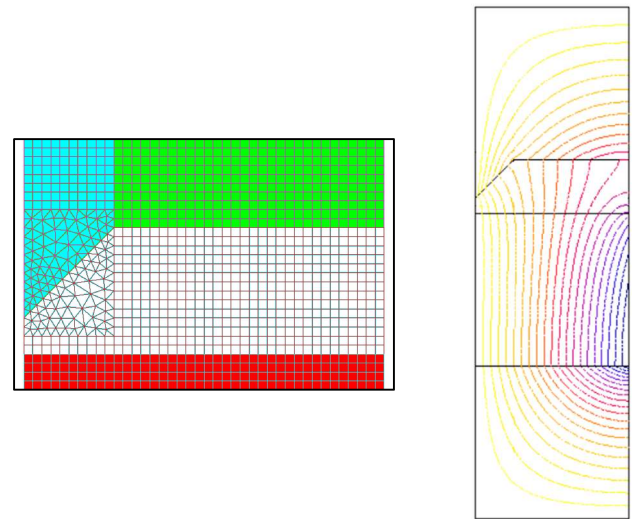
(a) FE mesh of the region of interest
