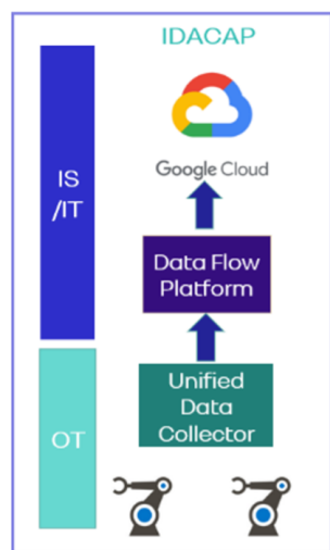
Figure 8. IDACAP architecture.
