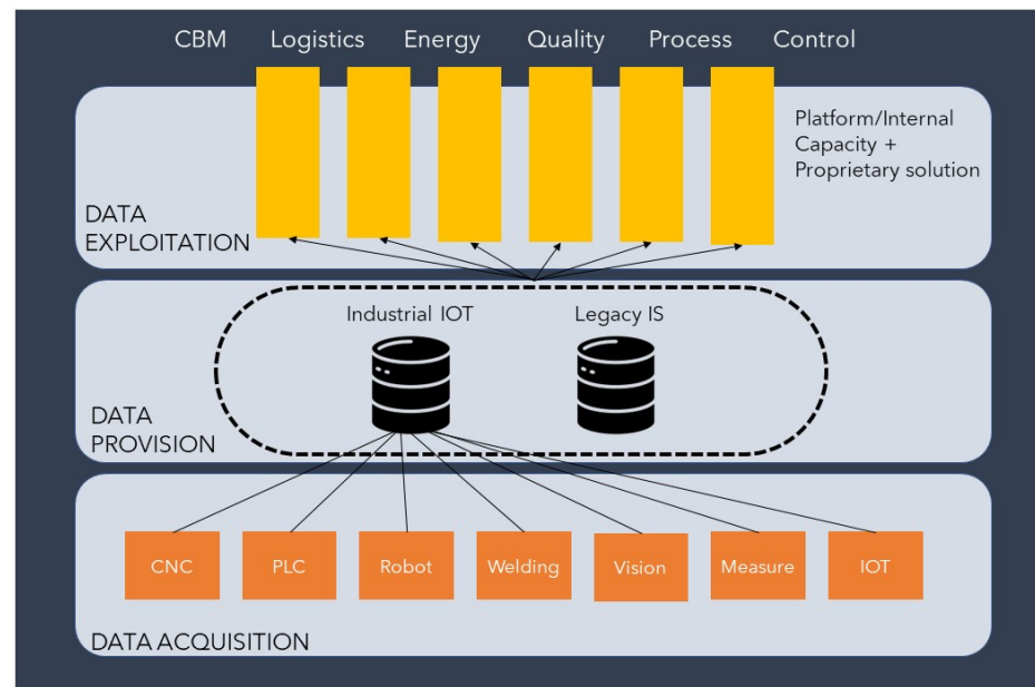
Figure 7. IDACAP architecture.
