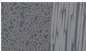
Fig. 7 Micrographic section in the section of a composite [0/90]
