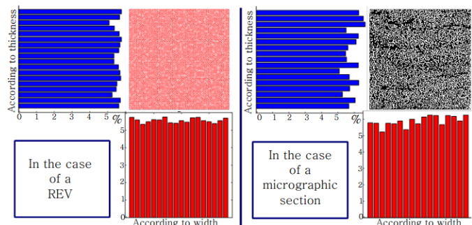
Fig. 9 Fiber distribution
