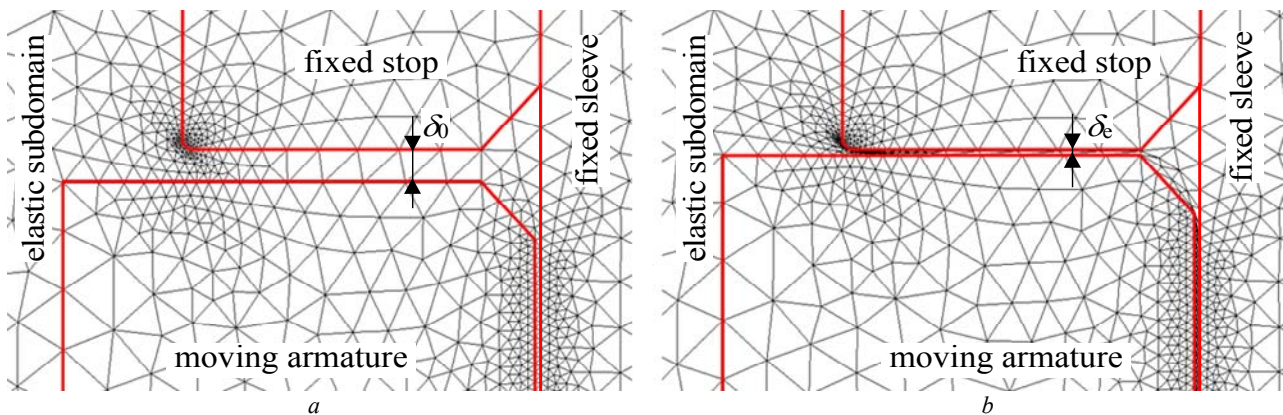
Fig. 7. A fragment of the calculation domain covered with a triangular mesh: a – armature in the initial position; b – armature in the end position
