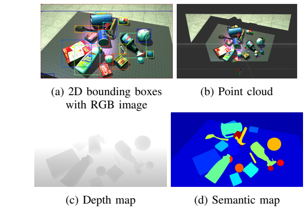
Fig. 1: Examples of annotations proposed for the dataset generation thanks to our Gazebo's plugin called PickSim.
