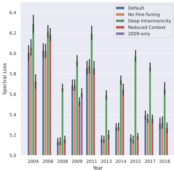
Fig. 2. Systems evaluation on the MAESTRO test set, broken down by recording environments. Measured by mean and standard deviation values of the multi-resolution spectral difference (as presented in Section 3.4) with the original recordings. Low loss value indicates better reconstruction quality.
