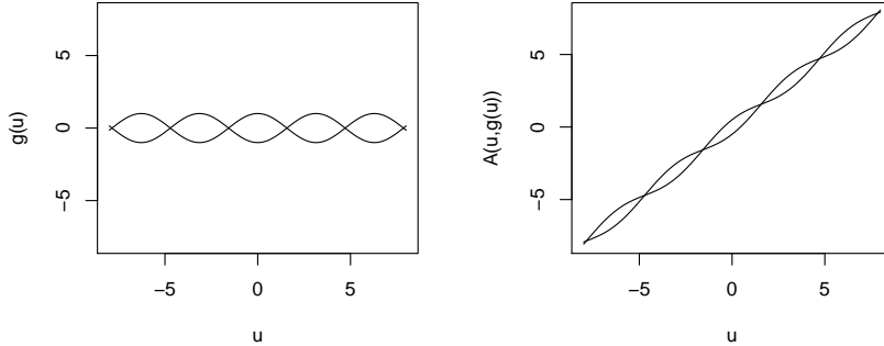
Figure 4: Left: support of S_0 and S_1 when \gamma = 1 . Right: support of X_0 and X_1 when \gamma = 1 .
