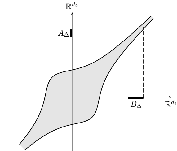
Figure 2: Illustration of (H1) and \mathcal{A}_1 for a non-compact support. As A_\Delta goes to infinity and becomes thinner, so does B_\Delta .
