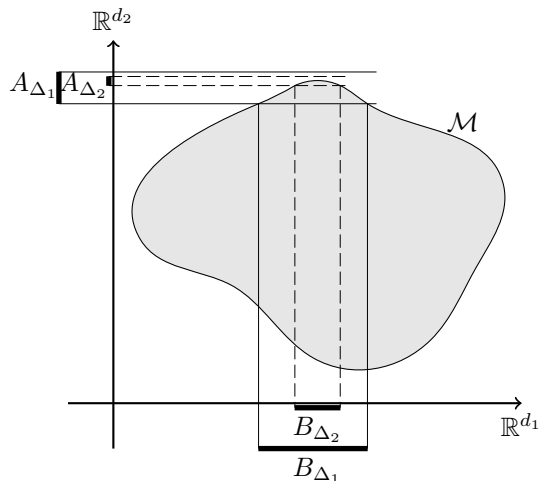
Figure 1: Illustration of (H1) and \mathcal{A}_1 . As A_\Delta narrows on the “tip” of the support, B_\Delta can be taken smaller and smaller. This narrowing as A_\Delta tends to the extremal point of the support is why \mathcal{B}_1 holds for compact supports with strictly convex convex hull.
