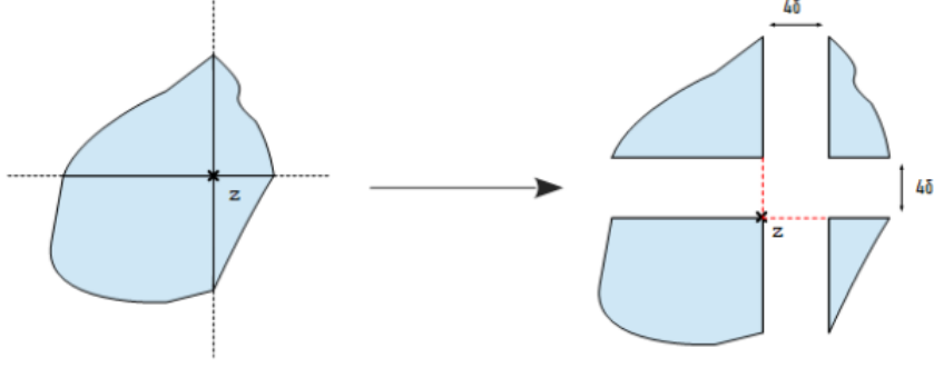
Figure 3: Transforming \mathcal{M} into a set \mathcal{M}' \in \mathcal{B}_1 \cap \mathcal{B}_2
