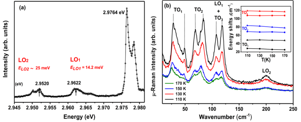
Fig. 3. (a) \mu -PL spectrum at 5 K of an excitonic doublet (splitting of 2 meV) and LO phonon replicas of CsPbCl 3 . The energies of clearly appearing structures are also indicated. The energies of the LO phonons observed are given. The energy reference is the one of the main excitonic line in this doublet. (b) Micro-Raman spectra as a function of temperature with a continuous excitation at 514.5 nm. The inset shows the weak dependences of the Raman shifts with temperature (100 cm -1 corresponds to \approx 12.4 meV).
