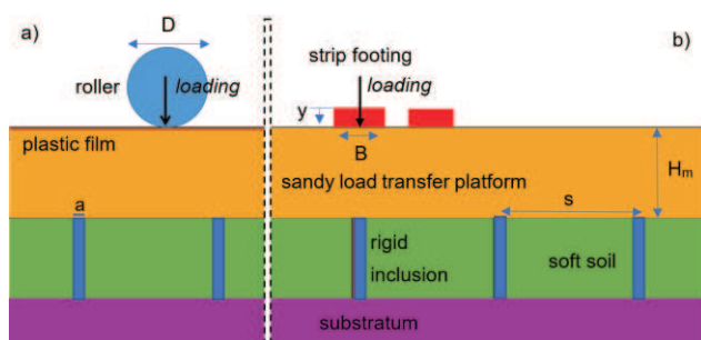
Fig. 1. 2D geometry of the physical model – a) roller in translation; b) static loading of a strip footing above a RI or between two RI.
