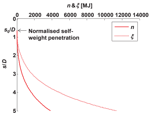
Fig. 3. Number of blows ( n ) and cumulative energy ( \xi ) at the prototype scale plotted against the normalised settlement of the monopile.
