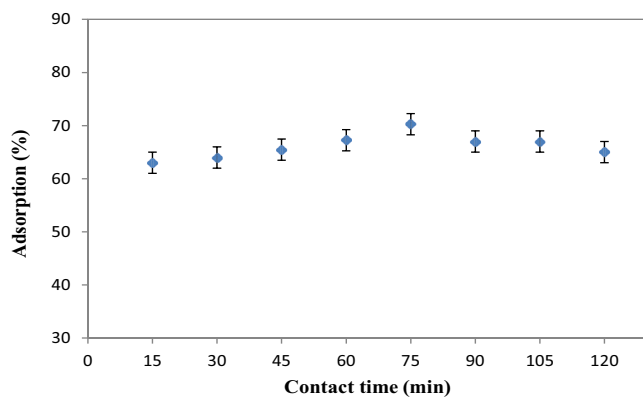
Fig. 4. Effect of contact time ( C_0 = 80 mg/L; m = 1.6 g; V = 50 mL; pH = 2.9; T = 298 K).
