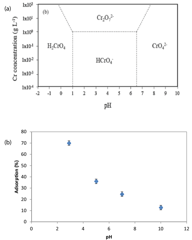
Fig. 3. Distribution of Cr(VI) species in water as a function of pH level and Cr(VI) concentration (a) and effect of pH ( C_0 = 80 mg/L; V = 50 mL; t = 75 min; T = 298 K) (b).
