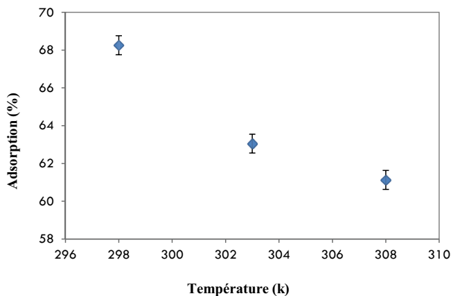
Fig. 5. Effect of temperature ( C_0 = 80 mg/L; m = 1.6 g; V = 50 mL; pH = 2.9; t = 75 min).
