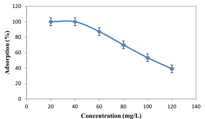
Fig. 6. Effect of initial Cr(VI) concentration ( m = 1.6 g; V = 50 mL; pH = 2.9; t = 75 min; T = 298 K).
