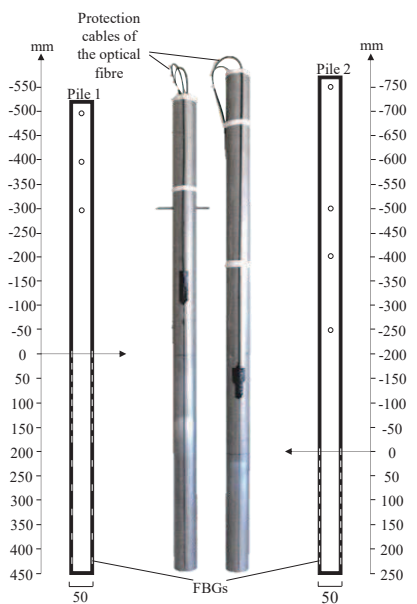
Fig. 1. Geometry of the instrumented model monopiles.
