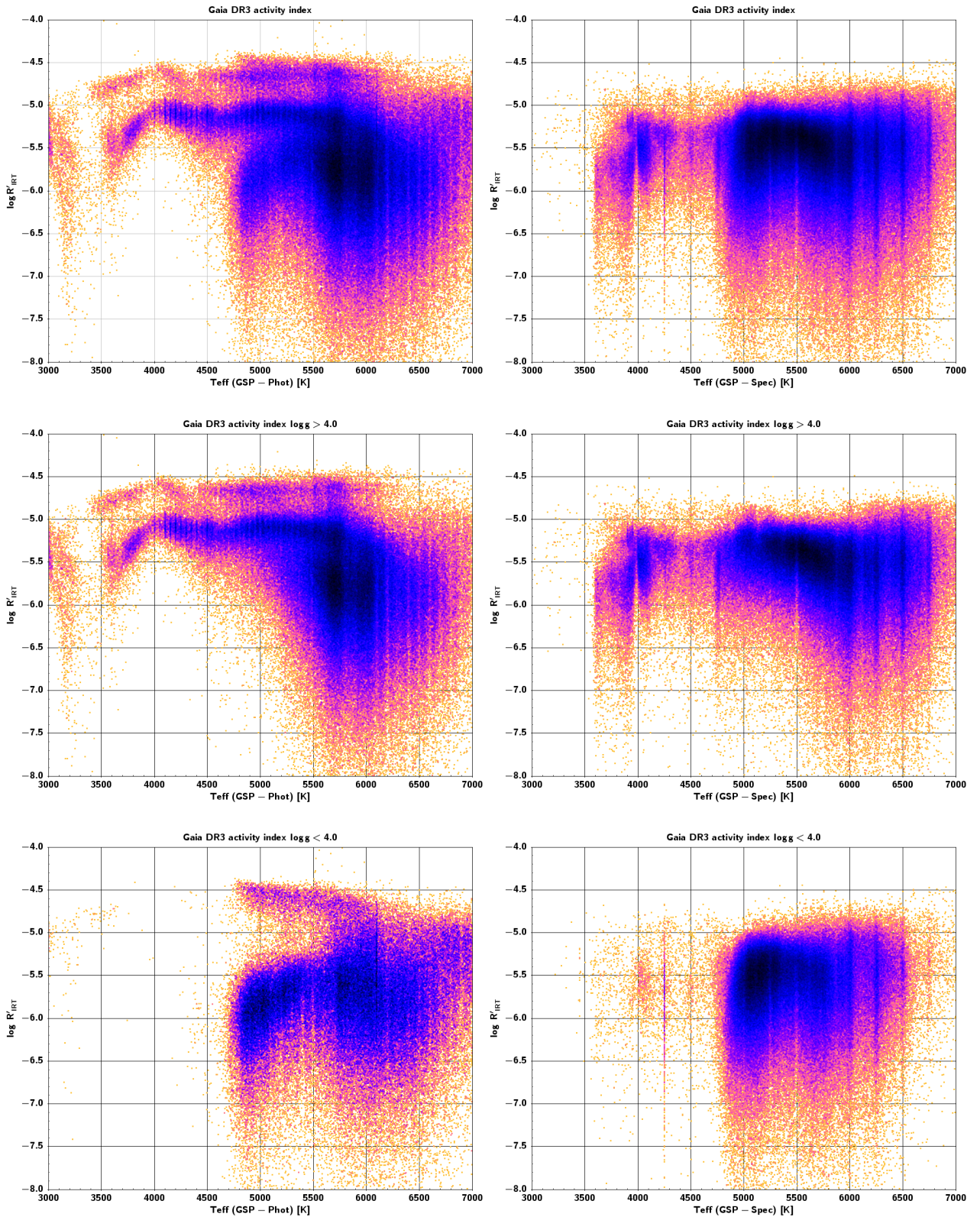
Fig. 3. Density plots of \log R'_{\text{IRT}} vs T_{\text{eff}} with input parameters from GSP-Phot (upper left panel) and from GSP-Spec (upper right panel). The same plots are repeated in the middle panels for \log g > 4.0 and in the lower panels for \log g < 4.0 .
