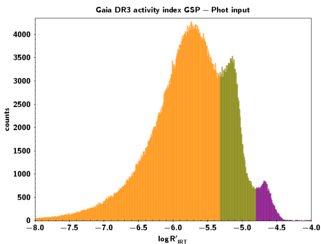
Fig. 4. Histogram of \log R'_{\text{IRT}} with input from GSP-Phot (bin size 0.01). The highest branch (VHA) is coloured in purple and has a lower limit between -4.8 and -5.0 , depending on T_{\text{eff}} . The second highest branch (HA) is coloured in green and has a lower limit between -5.3 and -5.5 , depending on T_{\text{eff}} . The remaining of the distribution (LA) is coloured in orange.
