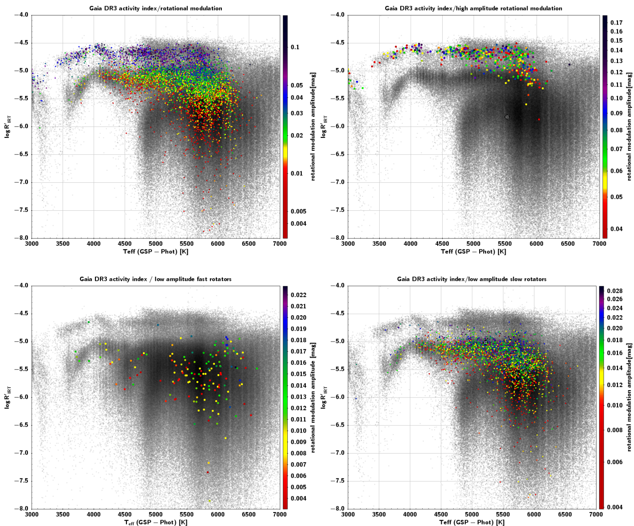
Fig. 10. \log R'_{\text{IRT}} vs T_{\text{eff}} density diagram from ( T_{\text{eff}} from GSP-Phot) with Gaia DR3 rotational modulation data overlaid (8171 sources in common). Top left panel: comparison with the whole rotational modulation dataset colour-coded according to the rotational modulation amplitude A . Top right panel: same as top left panel for just the high-amplitude rotator (HAR) branch. Bottom left panel: same as top left panel for just the low-amplitude fast-rotator (LAFR) branch. Bottom right panel: same as top left panel for just the low-amplitude slow-rotator (LASR) branch.
