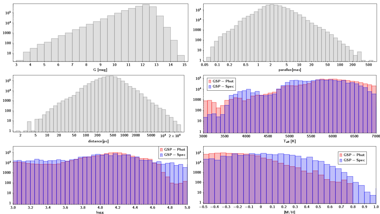
Fig. 1. Distribution in G , \varpi , distance (as derived by GSP-Phot Andrae 2022), T_{\text{eff}} , \log g , and [M/H] for the sources for which the activity index has been derived.
