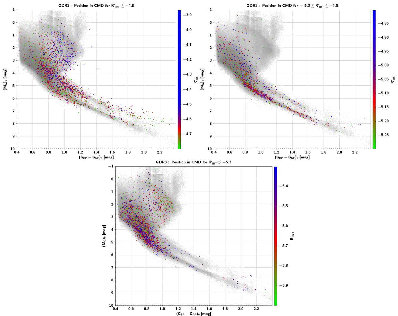
Fig. 6. Position in the CMD, corrected for interstellar extinction, of stars in the VHA (upper left panel), HA (upper right panel) and LA (lower panel) branches. Input APs are from GSP-Phot. The density plot of all sources for which the activity index has been derived is shown in grey on the background. The position of sub-samples of \sim 2000 stars per branch are shown in each panel, colour coded according to R'_{\text{IRT}} . See text for details.
