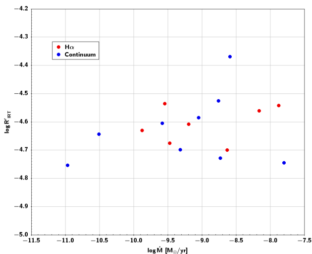
Fig. 8. Activity index ( \log R'_{\text{IRT}} ) vs accretion rate ( \log \dot{M} ) for selected sources. Red filled circles indicate accretion rates derived from the width of H\alpha at 10% of the peak by the Gaia-ESO survey (Lanzafame et al. 2015, and references therein). Blue filled circles indicate accretion rates derived from the excess continuum emission (see, e.g. Manara et al. 2015). See Table 2 for the sources of the accretion rate estimates.
