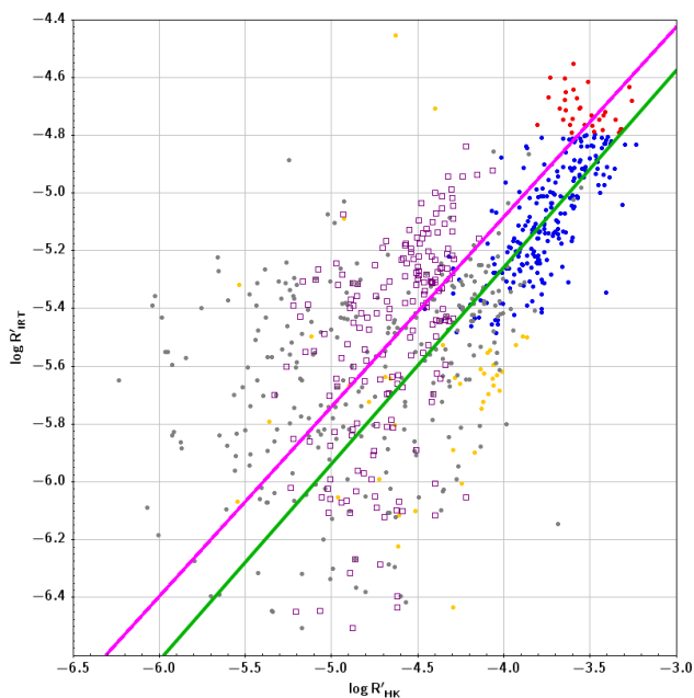
Fig. 7. Comparison of \log R'_{\text{IRT}} vs \log R'_{\text{HK}} obtained from ESO-FEROS archive spectra and with \log R'_{\text{HK}} from Boro Saikia et al. (2018). Stars with R'_{\text{IRT}} obtained from GSP-Phot input and placed in the HA-branch are plotted in blue, those in the VHA-branch in red, and those in the LA-branch in orange. Stars with R'_{\text{IRT}} obtained from GSP-Spec input are plotted in grey. The linear fit to data with GSP-Phot input is plotted in green (Eq. (8)). The comparison with R'_{\text{HK}} from Boro Saikia et al. (2018) is shown with open purple squares, and the corresponding linear fit with a purple line (Eq. (9)).
