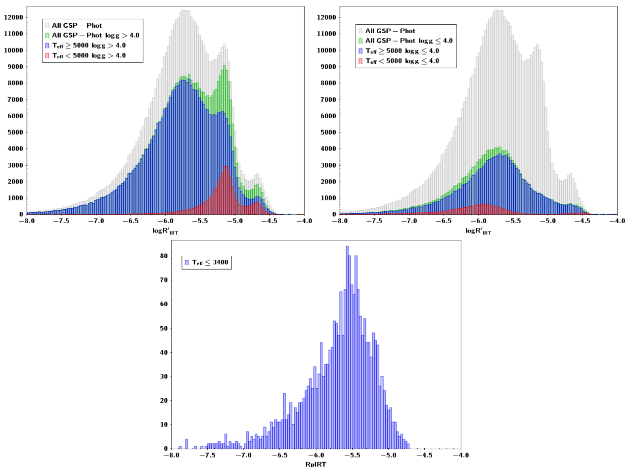
Fig. 9. \log R'_{\text{IRT}} histograms (bin size 0.03) for \log g > 4.0 (upper left panel) and \log g \leq 4.0 (upper right panel). In the upper panels, the distribution for T_{\text{eff}} \geq 5000 K and T_{\text{eff}} < 5000 K are compared with the global distributions. The distribution for T_{\text{eff}} \leq 3400 K (fully convective stars) is shown in the bottom panel. In order to extend the comparison to the very active branch on an homogeneous set, only results with GSP-Phot input are visualised.
