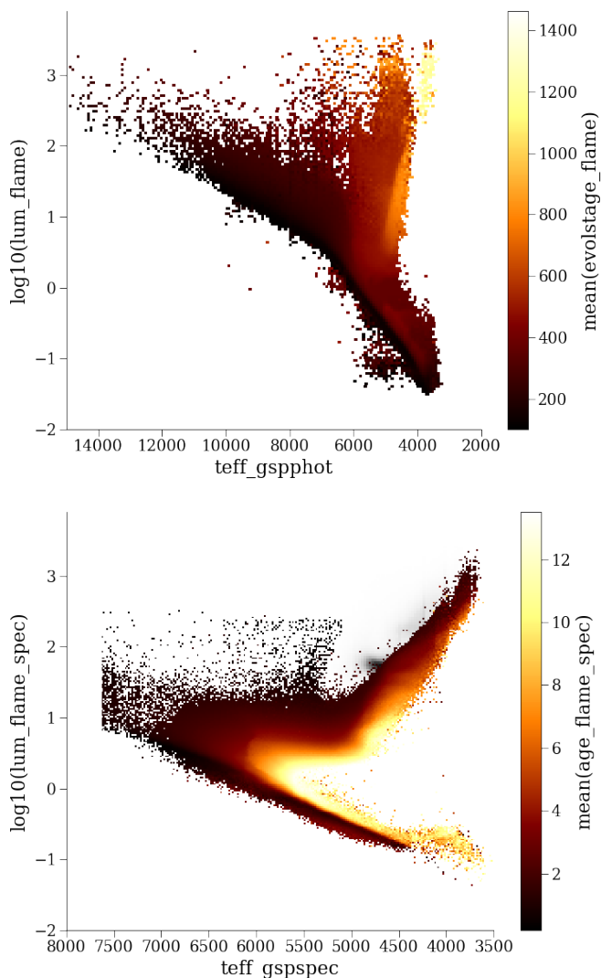
Fig. 24. HR diagrams colour-coded by FLAME parameters. Note that the colour-scale is linear and not a density plot. Top: \log_{10}(\text{lum\_flame}) versus \text{teff\_gspphot} colour-coded by \text{evolstage\_flame} for stars with relative parallax errors better than 10%. We have applied the recommended FLAME filter for giants. Lower: \log_{10}(\text{lum\_flame\_spec}) versus \text{teff\_gspspec} colour-coded by \text{age\_flame\_spec} for stars with \text{flags\_gspspec} like '0000000000000000%'. In the background the red clump can be seen in grey. These have no age values associated with them. Even though we have made selections on quality on certain parameters, there are still some artefacts that can be seen, such as the high-luminosity, low T_{\text{eff}} giants in the upper panel colour-coded by yellow, or the high-luminosity low mass main sequence stars in the lower panel. These artefacts can be removed by filtering on luminosity uncertainty, or requiring that the T_{\text{eff}} from both GSP-Spec and GSP-Phot agree to e.g. 300 K, or filtering on spectra SNR.
