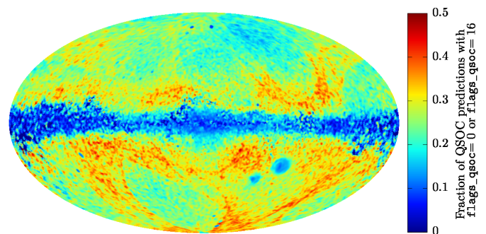
Fig. 25. Galactic sky distribution of the fraction of QSOC predictions that do not raise warning flags (i.e. \text{flags\_qsoc}=0 ), even if they are based on BP/RP spectra of lower quality (i.e. \text{flag\_Z\_BAD\_SPEC}=16 can be set). Fractions are computed within radii of 1^\circ over the whole celestial sphere.
