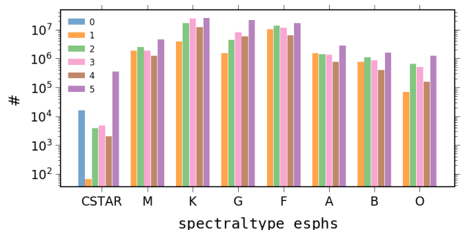
Fig. 13. Histogram of the distribution of spectraltypes_espsh which processed sources with G \leq 17.65 . A coloured distinction is made between the different values taken by the quality assessment flag (second digit of flags_espsh ). Usually the flag takes values ranging from 1 to 5, with the lower value indicating higher quality. However, for the CSTAR tag it can also be “0”.
