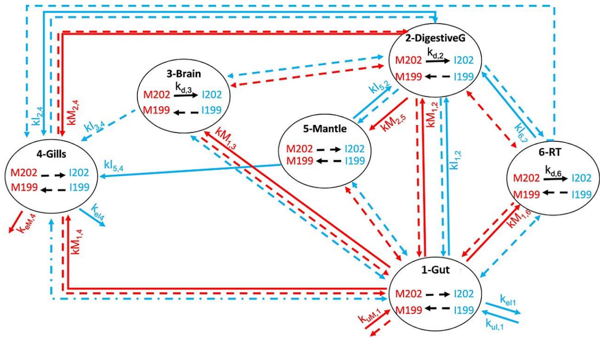
Figure 1. Modelling of in vivo mercury isotopes transformations and distribution in different organs of cuttlefish (gills, brain, mantle, digestive gland, intestine and remaining tissues). Dotted arrow: parameters estimated at very low values (<0.001), solid arrow: parameters estimated at high values (>0.001). M: MeHg, I:Hg(II), RT: remaining tissues.
