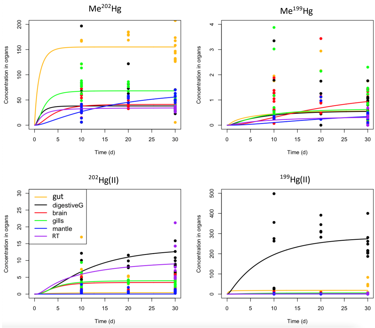
Figure S2. Adjustments of Hg species concentrations (ng.g -1 dry weight) measured in different organs of cuttlefish at different time (0, 10, 20 and 30 days), both pH conditions pooled, and based on the TK model. RT: remaining tissues.
