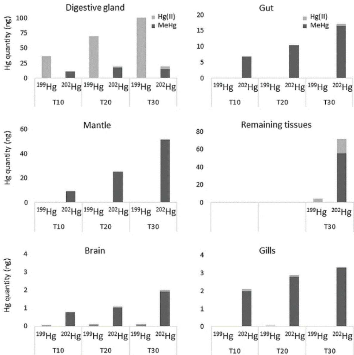
Figure 2. Quantity of Hg isotopes under inorganic (Hg(II)) and methylated forms (MeHg) measured in different organs of cuttlefish at 10, 20 and 30 days (except for the remaining tissues, just at 30 days).
