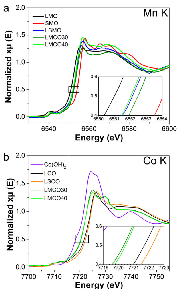
Figure 2. (a) Mn K-edge XANES spectra of powders: LMO , LSMO , LMCO30 , LMCO40 . The references for SMO is reported from Celorrio et al (CC-BY 4.0). 25 (b) Co-K-edge XANES spectra of powders: LCO , LSCO , LMCO30 , LMCO40 and \text{Co}(\text{OH})_2 . The inserts magnify the half-edge jump regions.
