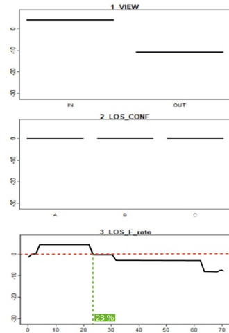
Figure 18. Random forest analysis.
