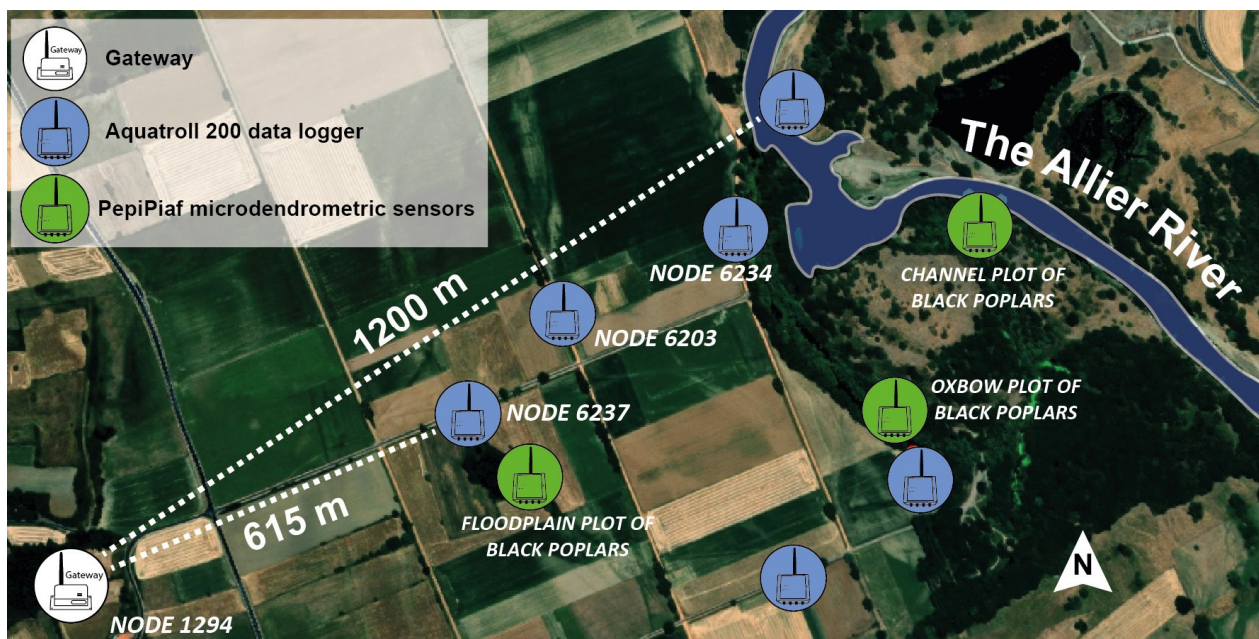
Figure 8. Location of sensors on the Auzon site (Image ©2023 Google, Images ©2023 CNES/Airbus).
