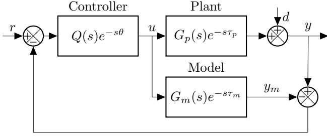
Fig. 1. The internal model control scheme
