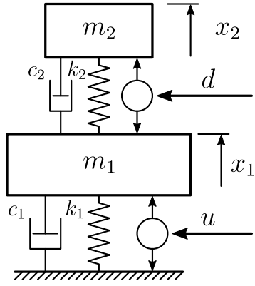
Fig. 2. Diagram of the controlled system
