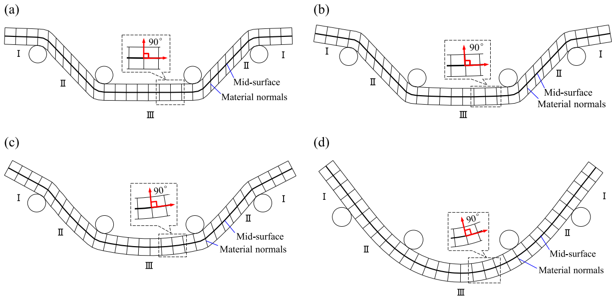
Fig. 3. The four-point bending simulation using Mindlin shell element with different transverse shell stiffness. (a) C_s = 0.001 \text{ N/mm} (b) C_s = 0.005 \text{ N/mm} (c) C_s = 0.025 \text{ N/mm} (d) C_s = 100 \text{ N/mm} . In these four tests, all the simulation settings and other material properties are the same. To visualize the transverse shear, the simulation results are post-processed in Matlab to plot the material normals.
