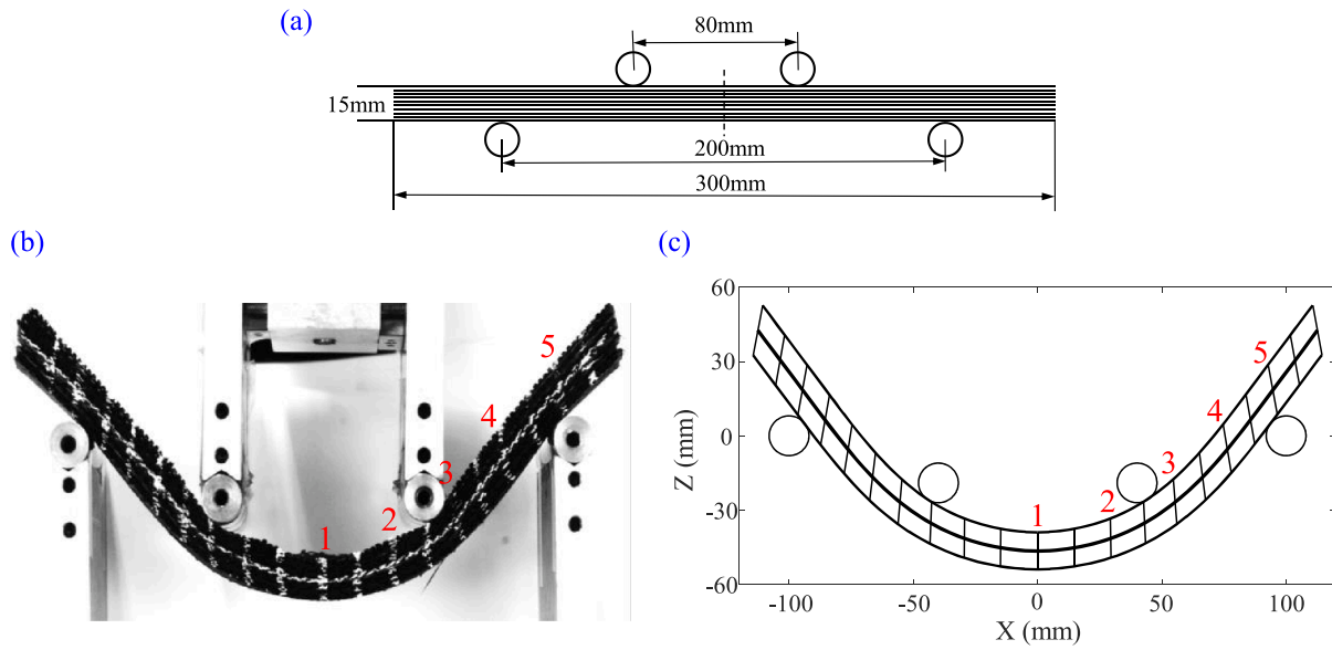
Fig. 10. Four-point bending of an 11-layer interlock fabric G1151. (a) Geometry. (b) Experimental results. In the experiment, the mid-surface and material normals are marked white. (c) Numerical results using resultant shell finite element calculation, and kinematic approach for the calculation of transverse shear. Five different positions 1–5 are marked to verify the correctness of numerical results.
