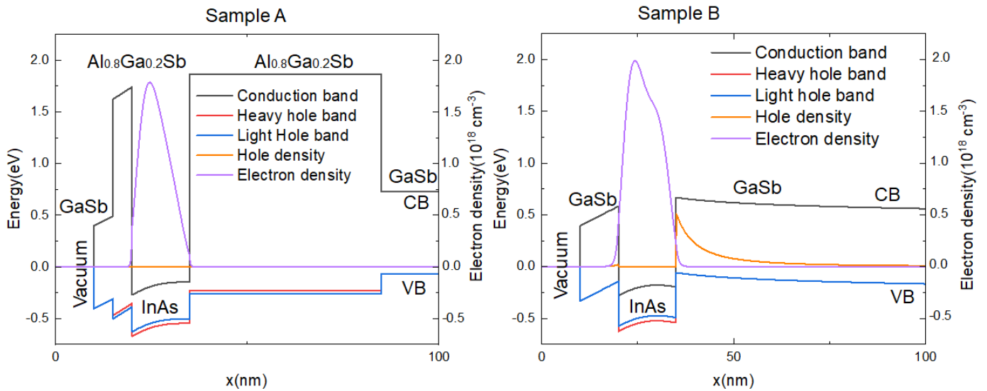
FIG. S1. Band diagram simulation of the 2DEG formed in sample A (left) and sample B (right) using Nextnano software [1]
