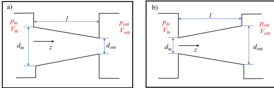
Figure 1: Design of a tapered microchannel with circular cross section. a) Converging tapered channel; b) Diverging tapered channel.
