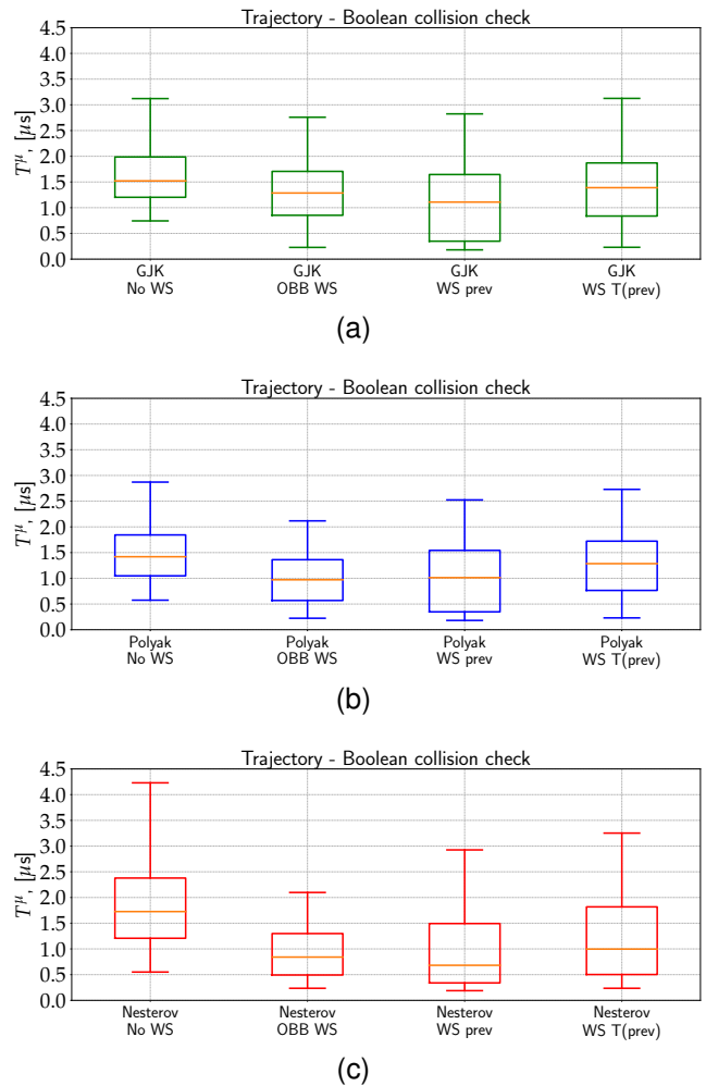
Fig. 12. Boolean collision checking of YCB objects' trajectories (see Fig. 13) for different warm-start strategies for (a) vanilla GJK, (b) Polyak-accelerated GJK, and (c) Nesterov-accelerated GJK (with normalization). In the three figures, WS is an abbreviation of warm-start . The No WS strategy signifies the algorithm is initialized with \mathbf{x}_0 = (1, 0, 0)^T . The OBB WS strategy uses the objects' current OBBs centers to compute \mathbf{x}_0 . In both WS prev and WS T(prev) , \mathbf{x}_0 is computed using GJK or EPA's previous solution, when this solution is available ( i.e. , when the previous collision problem was not discarded by the broadphase). Contrary to WS prev , WS T(prev) corrects the previous solution using the relative displacement of the shapes between the two considered time steps.
