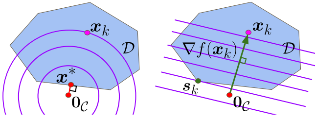
Fig. 3. Computing a support vector s_k in direction \nabla f(\mathbf{x}_k) on convex set \mathcal{D} . We illustrate with the example of distance computation. On the left, we draw the Minkowski difference \mathcal{D} of which point of minimum norm (MNP) is \mathbf{x}^* i.e. \mathbf{x}^* is the projection of \mathbf{0}_C onto \mathcal{D} , \mathbf{x}^* = \text{proj}_{\mathcal{D}}(\mathbf{0}_C) . The iterate at iteration k of the FW algorithm is \mathbf{x}_k . In purple we draw the level sets of the function f(\mathbf{x}) = \|\mathbf{x}\|^2 . On the right, we draw in purple the level sets of the linearization of f at iterate \mathbf{x}_k , h_k . The first step of the FW algorithm is to compute support vector s_k in the direction of \nabla f(\mathbf{x}_k) (green arrow), s_k \in S_{\mathcal{D}}(\nabla f(\mathbf{x}_k)) . In the second step of the FW algorithm, we compute \mathbf{x}_{k+1} as a convex combination of \mathbf{x}_k and s_k i.e. \mathbf{x}_{k+1} is a point on the segment [\mathbf{x}_k, s_k] .
