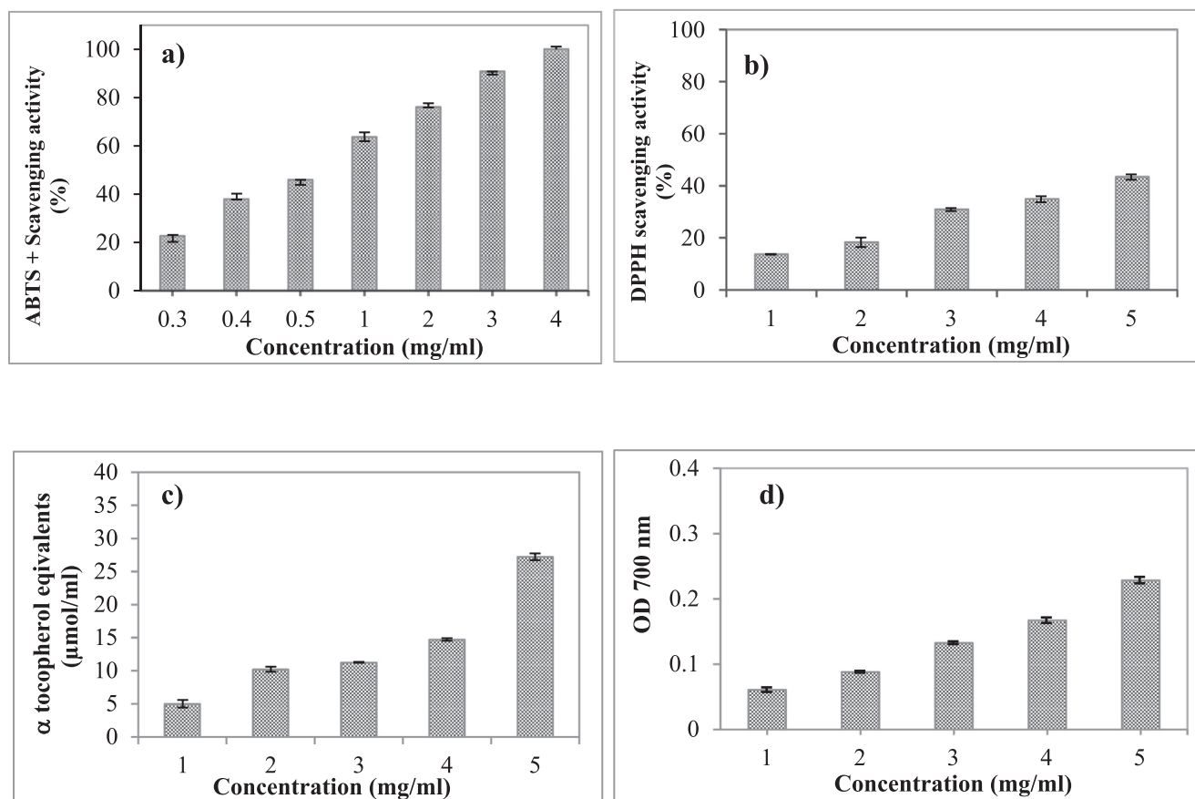
Fig. 4. Antioxidant activities of European skin gelatin (ESG) a) 2,2'-azino-bis (3-ethylbenzothiazoline-6-sulfonic acid) (ABTS) radical scavenging activity; b) 2,2-diphenyl-1-picryl-hydrazyl-hydrate (DPPH) free radical scavenging method; c) total antioxidant activity and d) reducing power.
