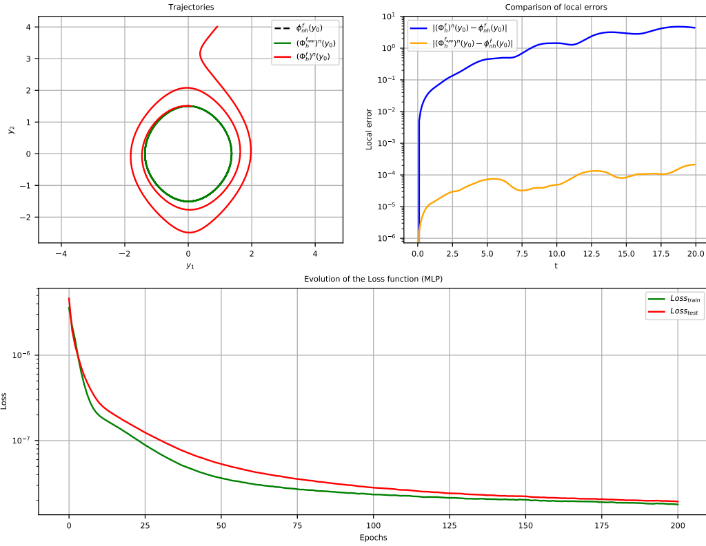
Figure 4: Comparison between Loss decays (green: Loss_{Train} , red: Loss_{Test} ), trajectories (dashed dark: exact flow, red: numerical flow with f , green: numerical flow with f_{app}(\cdot, h) ) and local error (blue: exact flow and numerical flow with f , yellow: exact and numerical flow with f_{app}(\cdot, h) ) for the nonlinear pendulum with Forward Euler method.
