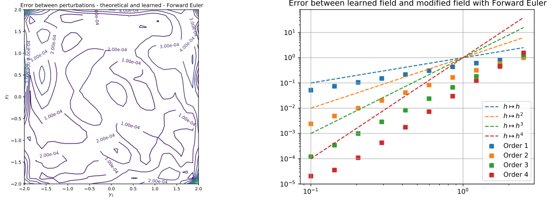
Figure 1: Forward Euler method. Left: Difference between \tilde{f}_h^4 and f_{app}(\cdot, h) for h = 0.1 . Right: Error between \tilde{f}_h^k and f_{app}(\cdot, h) for 1 \leq k \leq 4 .
