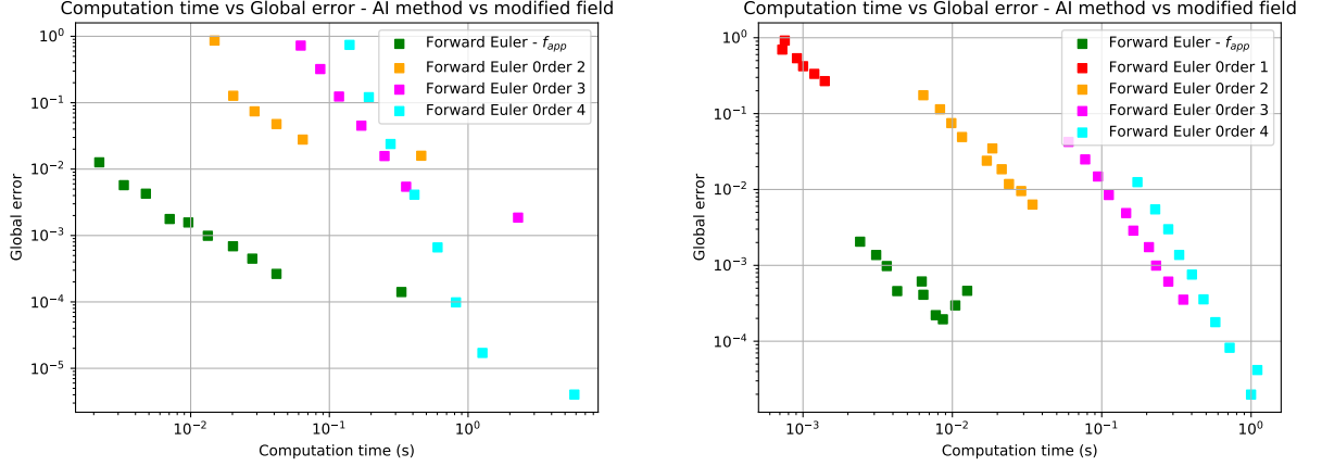
Figure 13: Computational time versus integration error for the Forward Euler method (red: with f , yellow: with \tilde{f}_h^2 , magenta: with \tilde{f}_h^3 , cyan: with \tilde{f}_h^4 , green: with f_{app}(\cdot, h) ). Left: Nonlinear Pendulum. Right: Rigid Body system.
