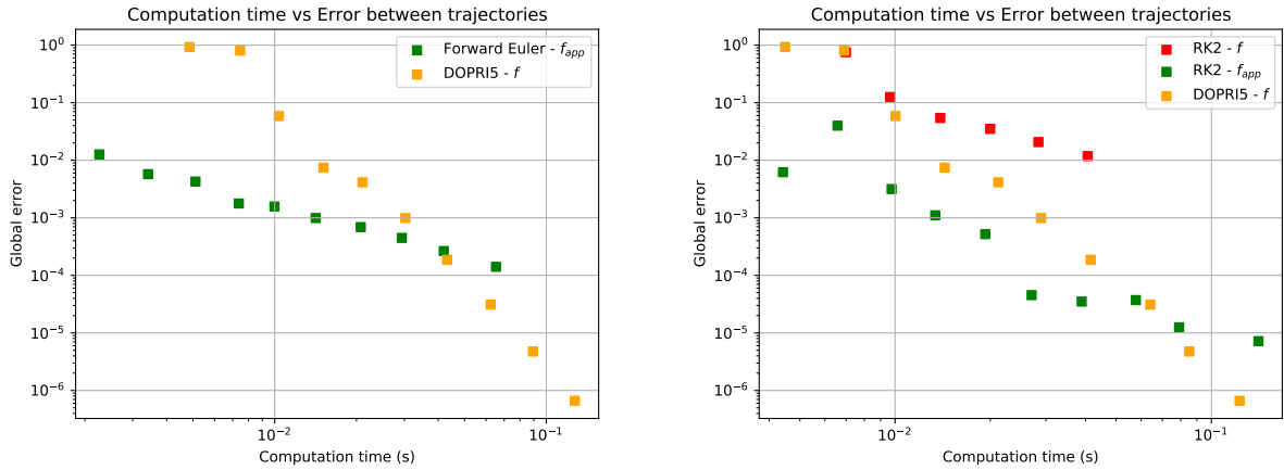
Figure 11: Comparison between computational time and integration error (red: numerical method with f , green: integration with f_{app}(\cdot, h) , yellow: integration with DOPRI5). Left: Nonlinear Pendulum with Forward Euler. Right: Nonlinear Pendulum with Runge-Kutta 2.
