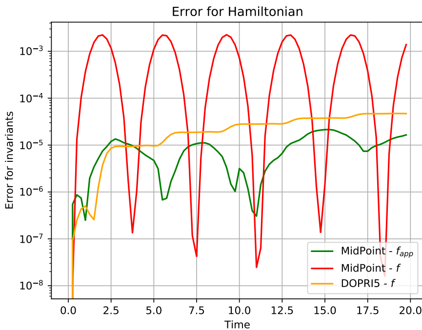
Figure 8: Evolution of the error between Hamiltonian H : y \mapsto (1 - \cos(y_2)) + \frac{1}{2}y_1^2 over the numerical flow and Hamiltonian at t = 0, H(y_0) .
