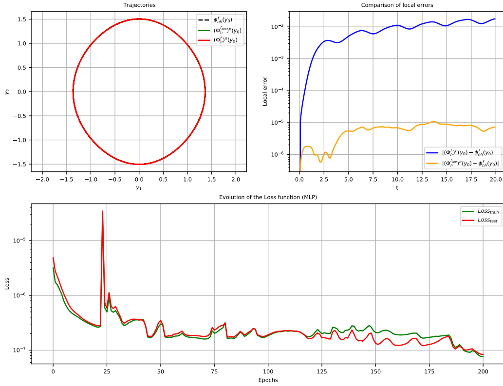
Figure 5: Comparison between Loss decays (green: Loss_{Train} , red: Loss_{Test} ), trajectories (dashed dark: exact flow, red: numerical flow with f , green: numerical flow with f_{app}(\cdot, h) ) and local error (blue: exact flow and numerical flow with f , yellow: exact and numerical flow with f_{app}(\cdot, h) ) for the nonlinear pendulum with Runge-Kutta 2 method.
