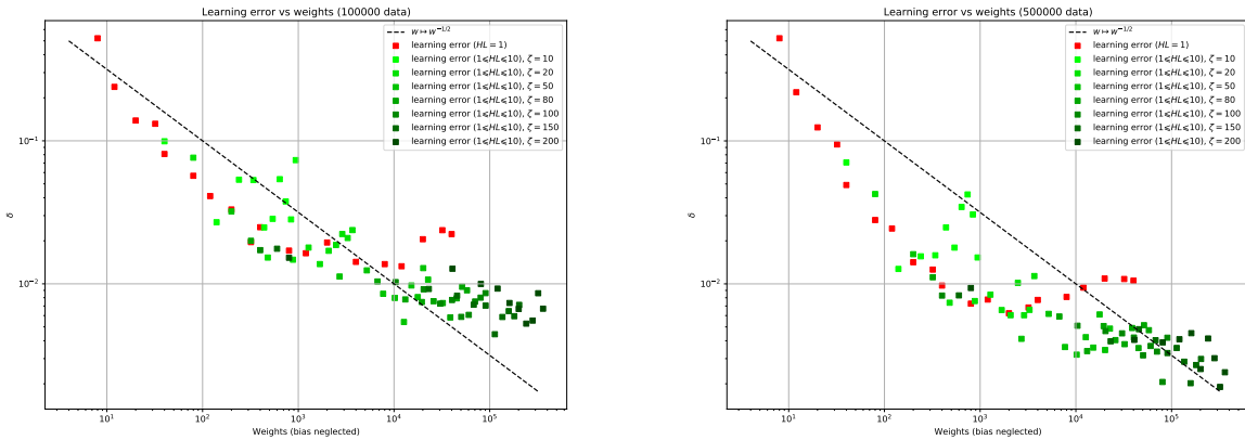
Figure 15: Learning error \delta versus number of parameters w in the neural network (number of neurons \zeta and hidden layers HL ). Shallow network is plot with red points whereas deep network is plot with green points (light green for 10 neurons to dark green for 200 neurons). Bias are neglected. Learning error is plot for 100 000 data (left) and 500 000 data (right). 200 epochs are used. [h^-, h^+] = [10^{-2}, 10^{-1}] . The curve of w \mapsto w^{\frac{1}{2}} has been added for comparison purposes.
