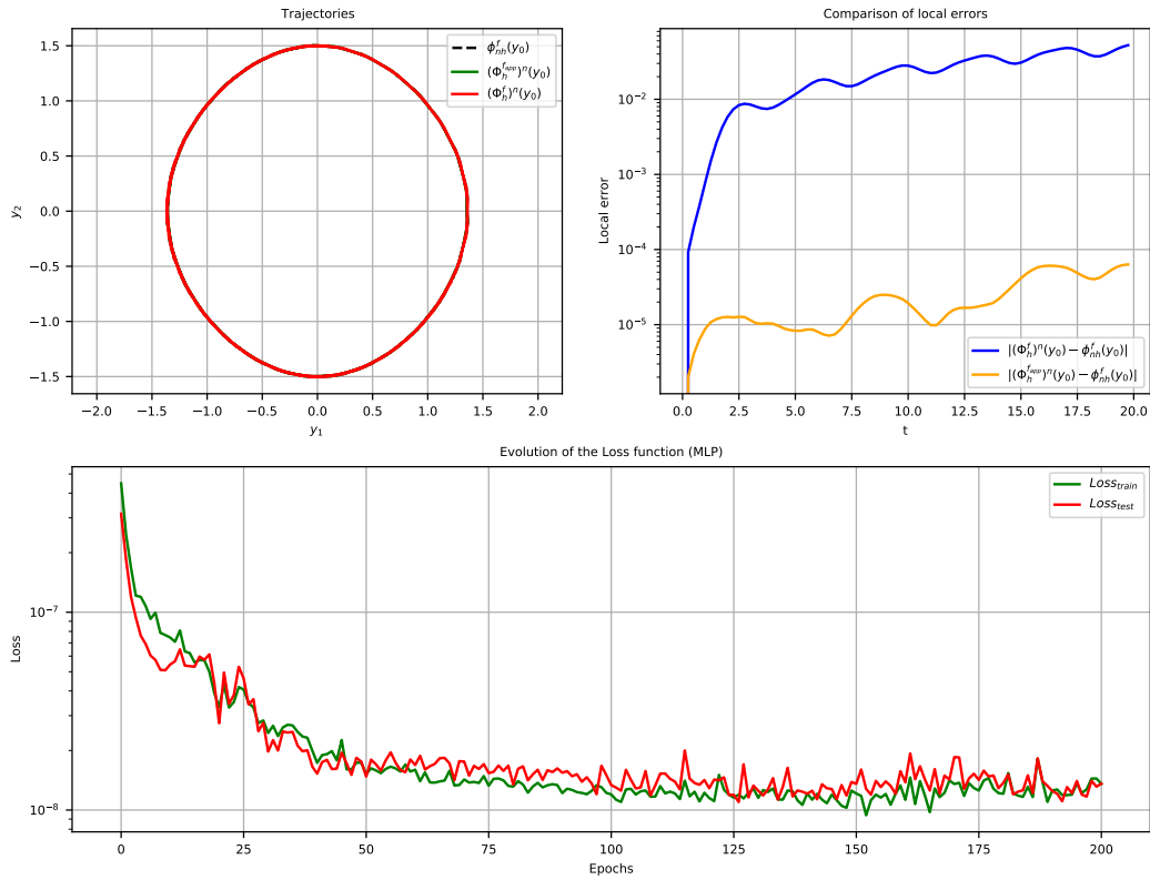
Figure 7: Comparison between Loss decays (green: Loss_{Train} , red: Loss_{Test} ), trajectories (dashed dark: exact flow, red: numerical flow with f , green: numerical flow with f_{app}(\cdot, h) ) and local error (blue: exact flow and numerical flow with f , yellow: exact and numerical flow with f_{app}(\cdot, h) ) for the nonlinear pendulum with midpoint method.
