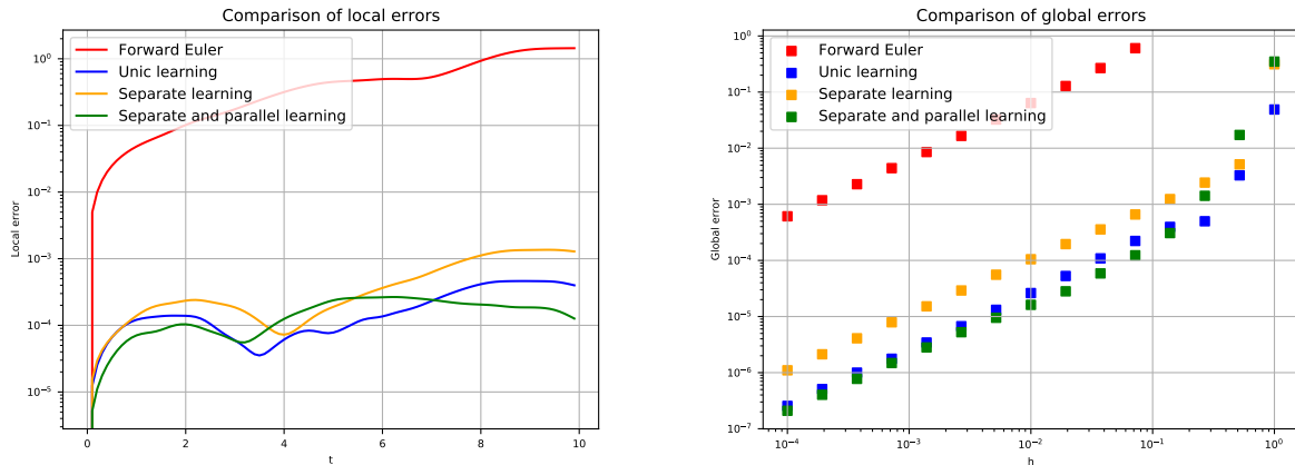
Figure 14: Comparison between forward Euler, traditional and alternative method for simple pendulum. Left: Comparison of local errors. Right: Comparison of integration errors.
