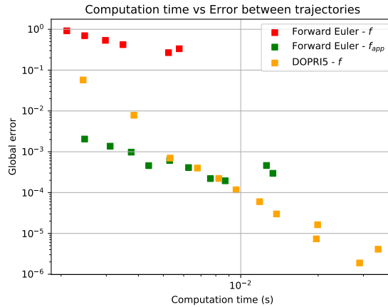
Figure 12: Comparison between computational time and integration error (red: numerical method with f , green: integration with f_{app}(\cdot, h) , yellow: integration with DOPRI5) for Rigid Body system with Forward Euler method.
