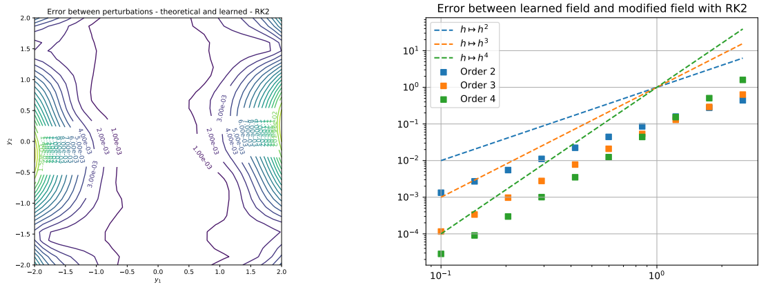
Figure 2: Runge-Kutta 2 method. Left: Difference between \tilde{f}_h^4 and f_{app}(\cdot, h) for h = 0.1 . Right: Error between \tilde{f}_h^k and f_{app}(\cdot, h) for 1 \leq k \leq 4 .
