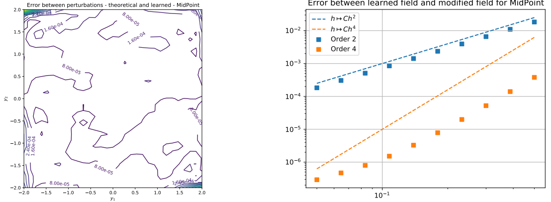
Figure 3: Midpoint method. Left: Difference between \tilde{f}_h^4 and f_{app}(\cdot, h) for h = 0.05 . Right: Error between \tilde{f}_h^k and f_{app}(\cdot, h) for 1 \leq k \leq 4 . Note that owing to the structure of the modified field for midpoint method (see [8, 14]), terms for odd powers of h vanish.
