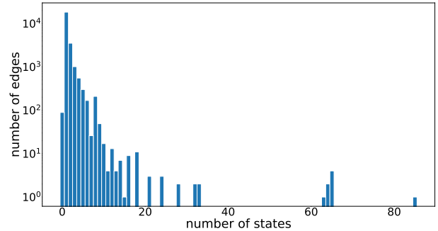
Fig. 4: The distribution of number of pipeline states.
