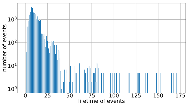
Fig. 5: The distribution of events lifetime.
