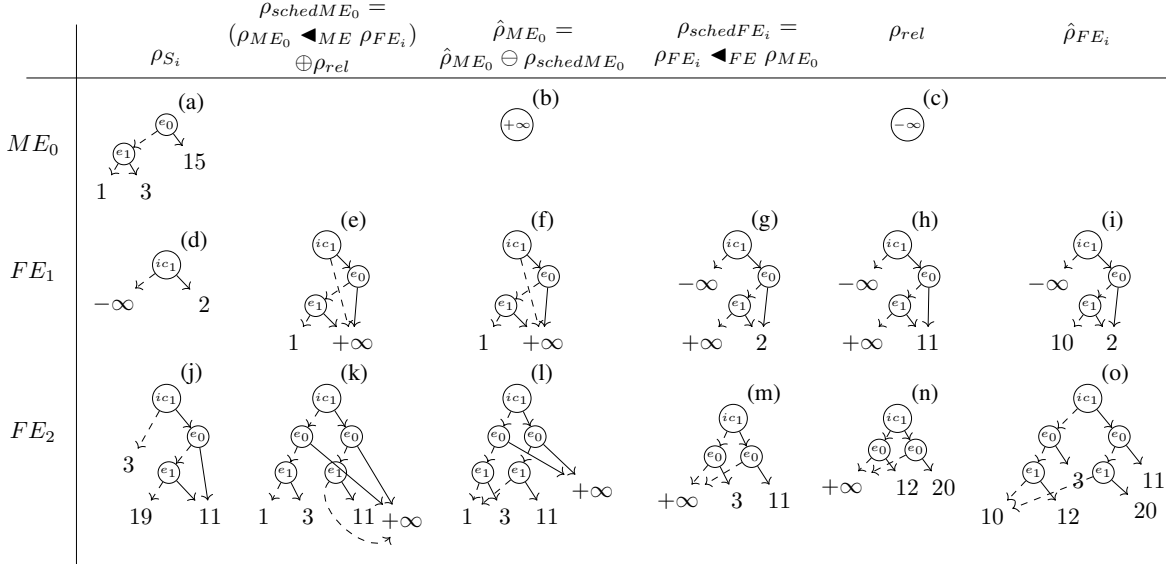
Fig. 3: Batch bus scheduling with XDDs.
