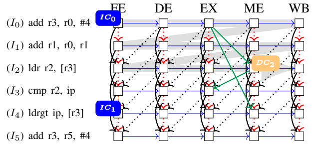
Fig. 1: XG model of an instruction sequence.
