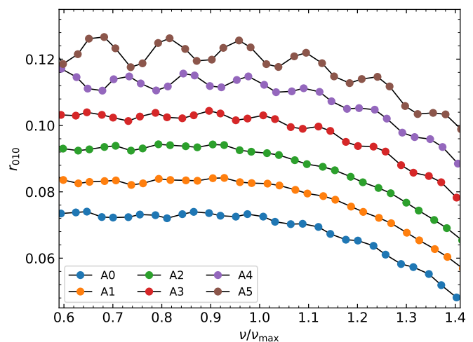
Fig. 2. r_{010} ratios for the 1.4M_\odot models A0 to A5 all at X_c = 0.10 . All curves have a mean of about 0.07, and all but A0 are gradually shifted by 0.01 for clarity.
