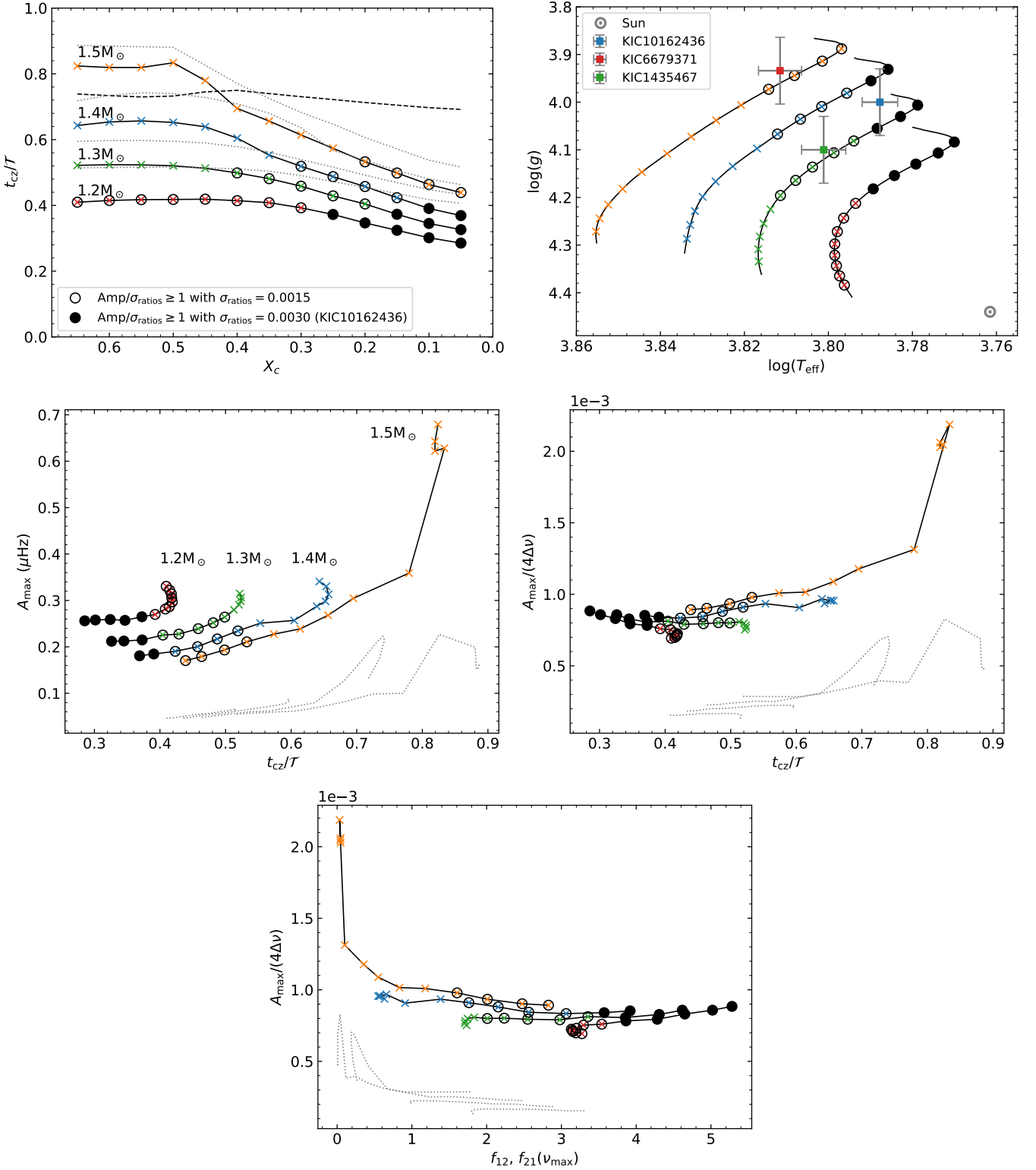
Fig. 8. Detectability of the signature in the r_{010} ratios for different quantities. The open and black circles show that the signature of the BSCZ glitch has an amplitude, Amp = A_{\text{max}}f_{12/21}(\nu_{\text{max}})/(4\Delta\nu) , that is larger than 0.0015 and 0.0030 (the mean uncertainty of the r_{010} ratios of 16 Cyg A and KIC10162436 around \nu_{\text{max}} ), respectively. Top left: Ratio of the acoustic radius of the BSCZ ( t_{cz} ) over the total acoustic radius ( \mathcal{T} ) for models with masses between 1.2 and 1.5M_{\odot} and \xi_{PC} = 2 . The dashed line represents the position of the iron/nickel convective zone induced by their accumulations due to radiative accelerations for a 1.5M_{\odot} model. Top right: Associated evolutionary tracks in a Kiel diagram. Middle left: Amplitudes A_{\text{max}} according to the ratio of the acoustic radius of the BSCZ ( t_{cz} ) over the total acoustic radius ( \mathcal{T} ) for the same models. Middle right: Amplitudes A_{\text{max}}/(4\Delta\nu) according to the ratio of the acoustic radius of the BSCZ ( t_{cz} ) over the total acoustic radius ( \mathcal{T} ) for the same models. Bottom: Amplitudes A_{\text{max}}/(4\Delta\nu) according to f_{12,21} at \tilde{\nu} = \nu = \nu_{\text{max}} . For the top left, middle and bottom panels, the dotted grey lines represent the same models with \xi_{PC} = 0 .
