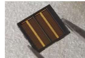
\mu TEG after assembly of the concentrator on the thermopile
