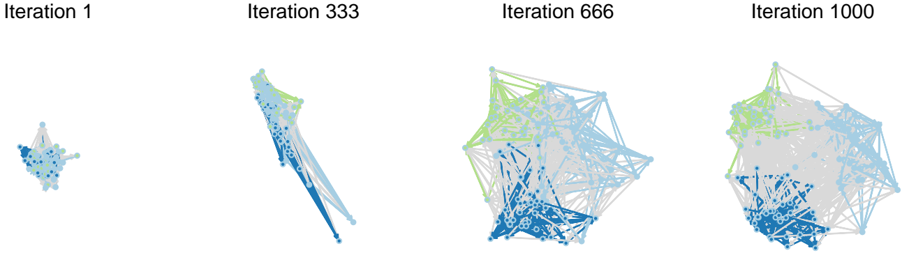
FIGURE 5 Evolution of the latent node positions during the training of Deep-LPTM.
