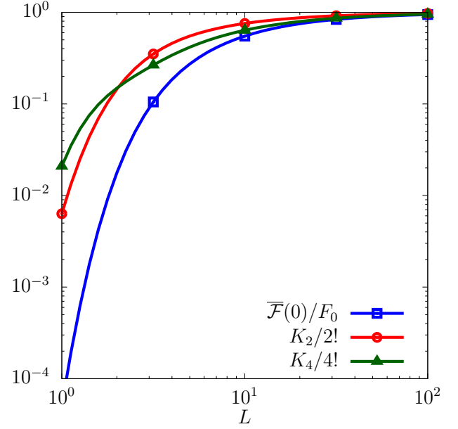
FIG. 15. Ratios \bar{\mathcal{F}}(0)/F_0 , K_2/2! and K_4/4! computed at various values of the normalized transverse size of the system, L = 2\pi R/\beta for the bounded system discussed in Sec. VI.
