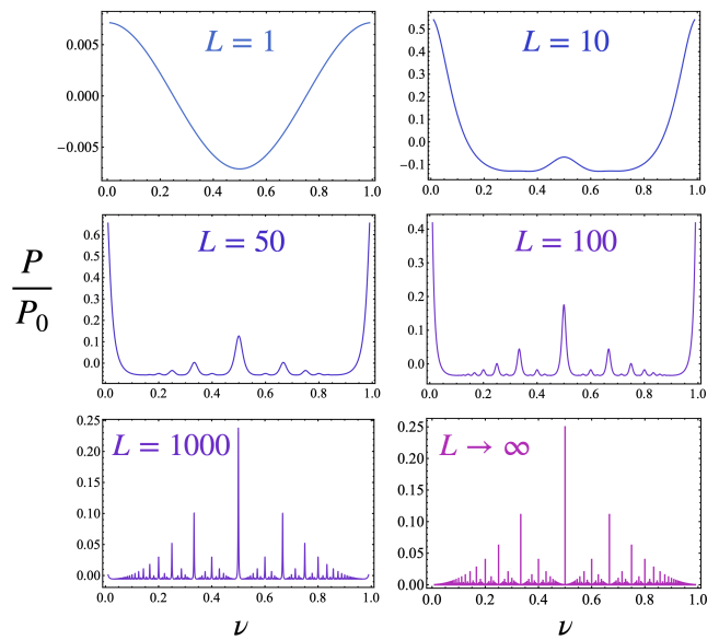
FIG. 4. Fractalization of thermodynamics of scalar particles on the ring under the imaginary rotation \Omega_I : pressure P , Eq. (31), shown in units of pressure P_0 for an infinite ring L \rightarrow \infty in the absence of rotation, Eq. (17), as a function of the normalized statistical angle \nu = \chi/(2\pi) \equiv \beta\Omega_I/(2\pi) for various (normalized) lengths L of the ring (30). The plots at finite values of L are given for the analytical behaviour (31) in terms of the Dedekind \eta function (29). The behaviour in the thermodynamic limit, L \rightarrow \infty , corresponds to the non-analytical fractal result (38) expressed via the Thomae function (15). The behaviour near the points \nu = 0 and \nu = 1 is not shown to preserve a convenient vertical scale.
