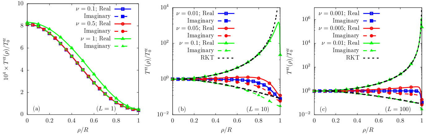
FIG. 11. Profiles of T^{tt}(\rho)/T_0^{tt} , represented with respect to the dimensionless radial coordinate \rho/R for a system enclosed within a cylindrical boundary located at R = \beta L/2\pi , with L = 1 (a), 10 (b), and 100 (c). The rotation parameter satisfies \nu L = 0.1 (blue squares), 0.5 (red circles), and 1 (green triangles). Solid and dashed lines and symbols denote profiles corresponding to real and imaginary rotation, respectively. The black dotted lines shown in panels (b) and (c) correspond to the RKT results (see text).
