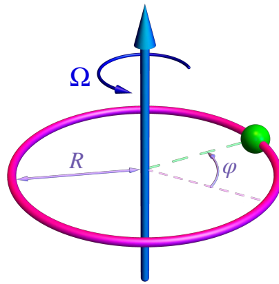
FIG. 3. Illustration of a particle on a ring of the radius R and the angular coordinate \varphi . The ring rotates with the angular velocity \Omega counterclockwise.
