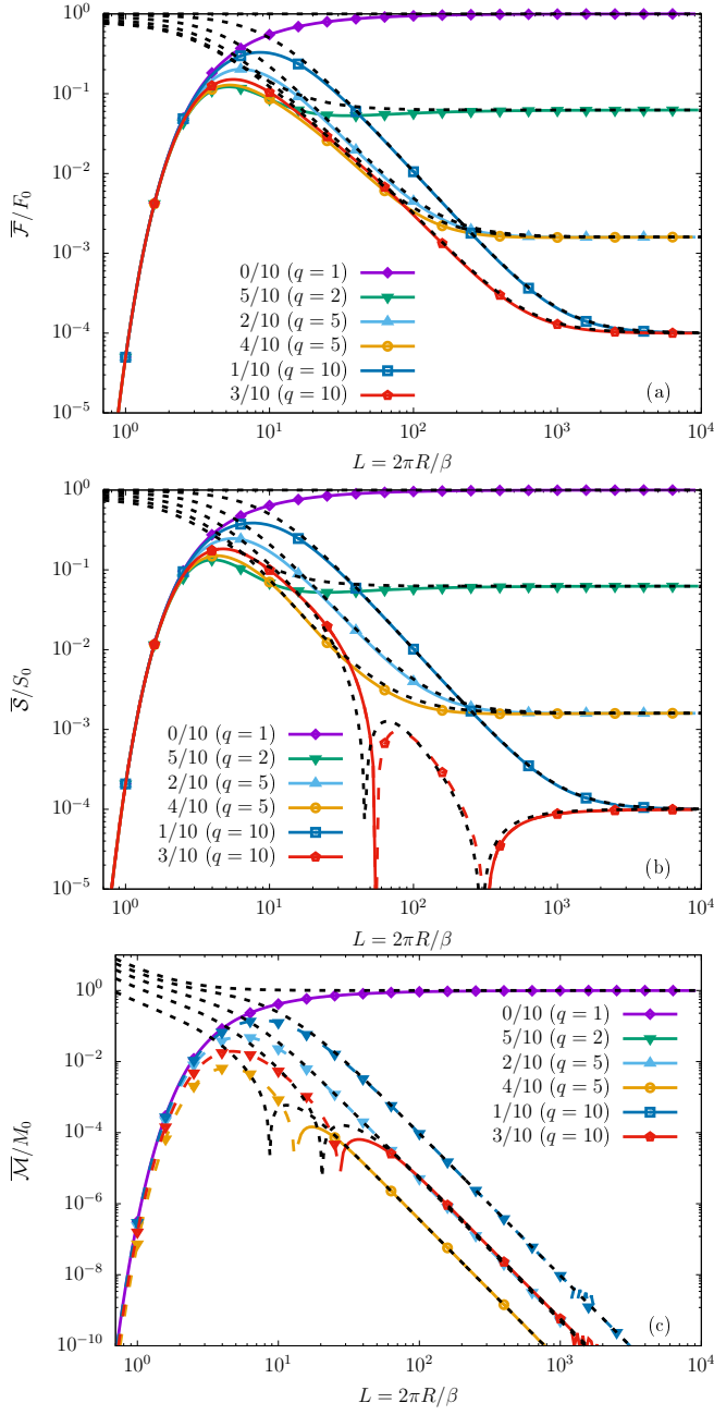
FIG. 14. Same as Fig. 13 for (a) \bar{\mathcal{F}}/F_0 , (b) \bar{\mathcal{S}}/S_0 and (c) \bar{\mathcal{M}}/M_0 .
