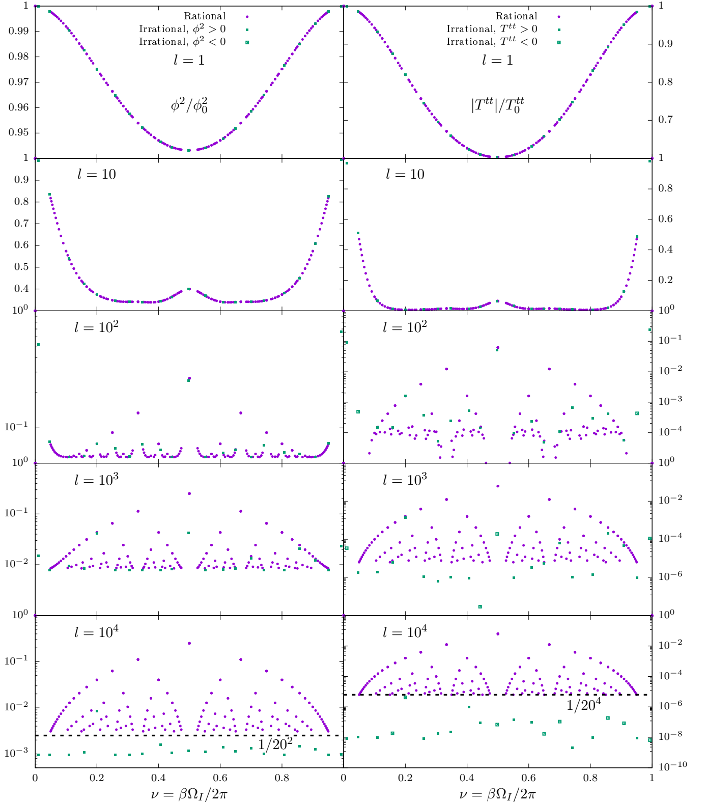
FIG. 9. Thermal expectation values of (left) \phi^2 normalized by \phi_0^2 = 1/12\beta^2 ; and (right) |T^{tt}| normalized by T_0^{tt} = \pi^2/30\beta^4 , shown with respect to the rotation parameter \nu = \beta\Omega_I/2\pi , for various values of the distance parameter l = 2\pi\rho/\beta from the axis of rotation of the cylinder. The purple circles correspond to the case when \nu = p/q is a rational number (we considered all irreducible fractions with 1 \leq q \leq 20 ). The green squares correspond to the irrational values \nu_j shown in Eq. (157). The empty symbols indicate the case when T^{tt} < 0 . The dashed line shown in the bottom panels (for l = 10^4 ) indicate the expected lower bounds (left) 1/q^2 and (right) 1/q^4 with q = 20 . This figure should be compared with Fig. 4 for particles in the ring: As the size of the cylinder grows, the thermodynamic expectation values in the cylinder get fractal features similar to the fractalization of thermodynamics of scalar particles in the ring.
