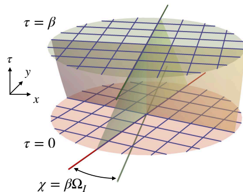
FIG. 1. The rotwisted boundary conditions (8) characterized by the statistical angle (7) produced by the imaginary angular velocity \Omega_I .
