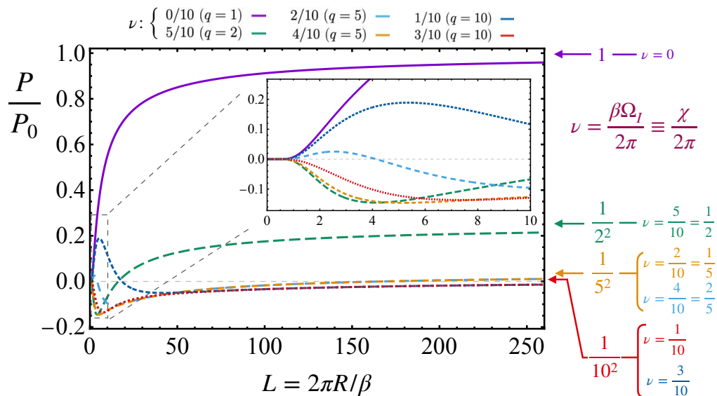
FIG. 6. The thermal contribution to the pressure, P \equiv P(L, \nu) , as a function of the (normalized) length of the ring L = 2\pi R/\beta for various (normalized) statistical angles \nu = \chi/(2\pi) with the rational values \nu = n/10 at n = 0, 1, \dots, 5 . The pressure is normalized to its value P_0 , Eq. (17), for a nonrotating ring, in the infinite-volume limit, L \rightarrow \infty . For rational \nu , the pressure (35), (38) in the infinite-volume limit takes fractal values (shown by the arrows) dictated by the Thomae function (15). The inset shows the zoom in on the small-radius region.
