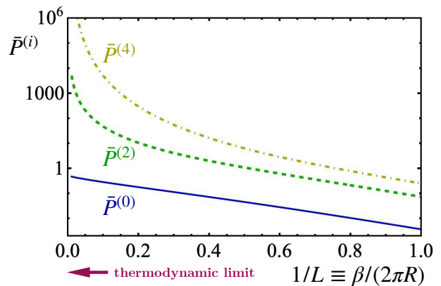
FIG. 5. The first three nonzero coefficients in the series (45) of pressure of the ring as a function of the (inverse) normalized radius 1/L . The direction of the thermodynamic limit is shown by the arrow.
