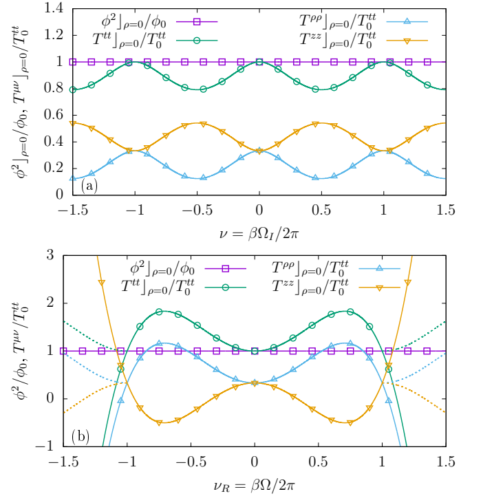
FIG. 7. The condensate \phi^2 and the components of the energy-momentum tensor T^{\mu\nu} on the axis of rotation of the cylinder, \rho = 0 , under (a) imaginary rotation with \nu \equiv \nu_I = \beta\Omega_I/2\pi and (b) real rotation with \nu_R = \beta\Omega/2\pi , normalized with respect to their values in the absence of rotation. All quantities under imaginary rotation are periodic ( \nu \rightarrow \nu + 1 ) in agreement with Eq. (10). The dashed lines extending in the region |\nu_R| > 1 indicate the expected behaviour if the components of T_{\mu\nu} were periodic with respect to \nu_R .
