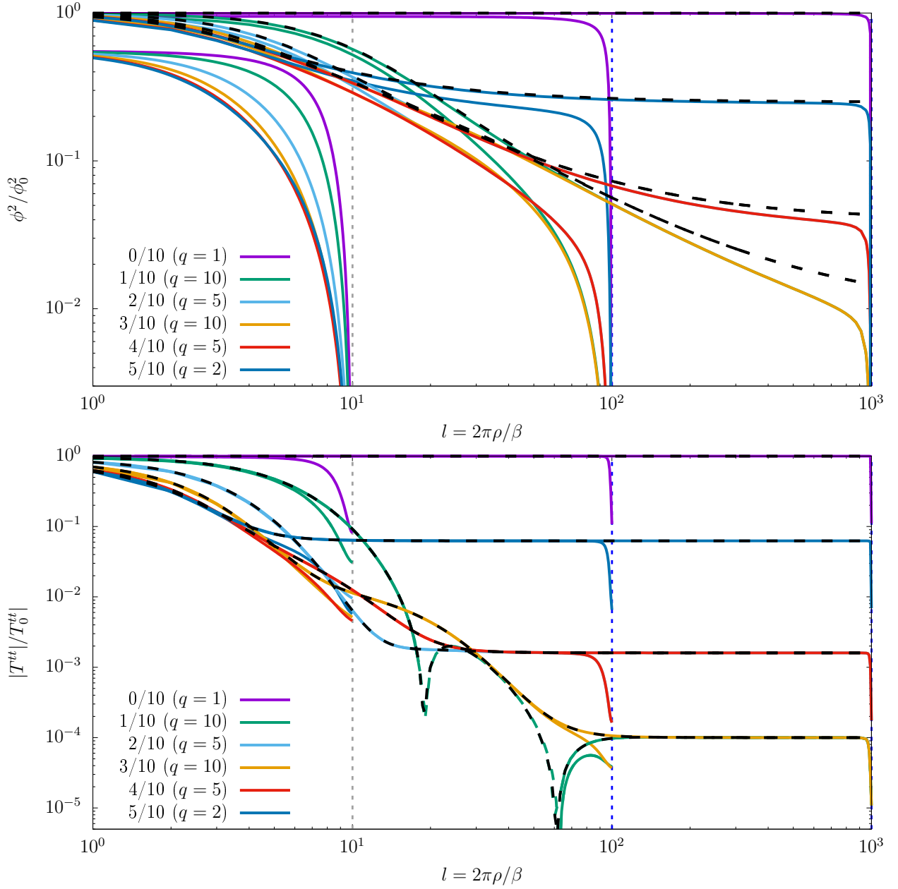
FIG. 10. Same as Fig. 8 for the case when the system is enclosed within cylindrical boundaries of three different sizes, shown using vertical dotted lines, located such that L = 2\pi R/\beta = 10, 100 and 1000 . The black dashed lines represent the results obtained in the unbounded case, shown in Fig. 8.
