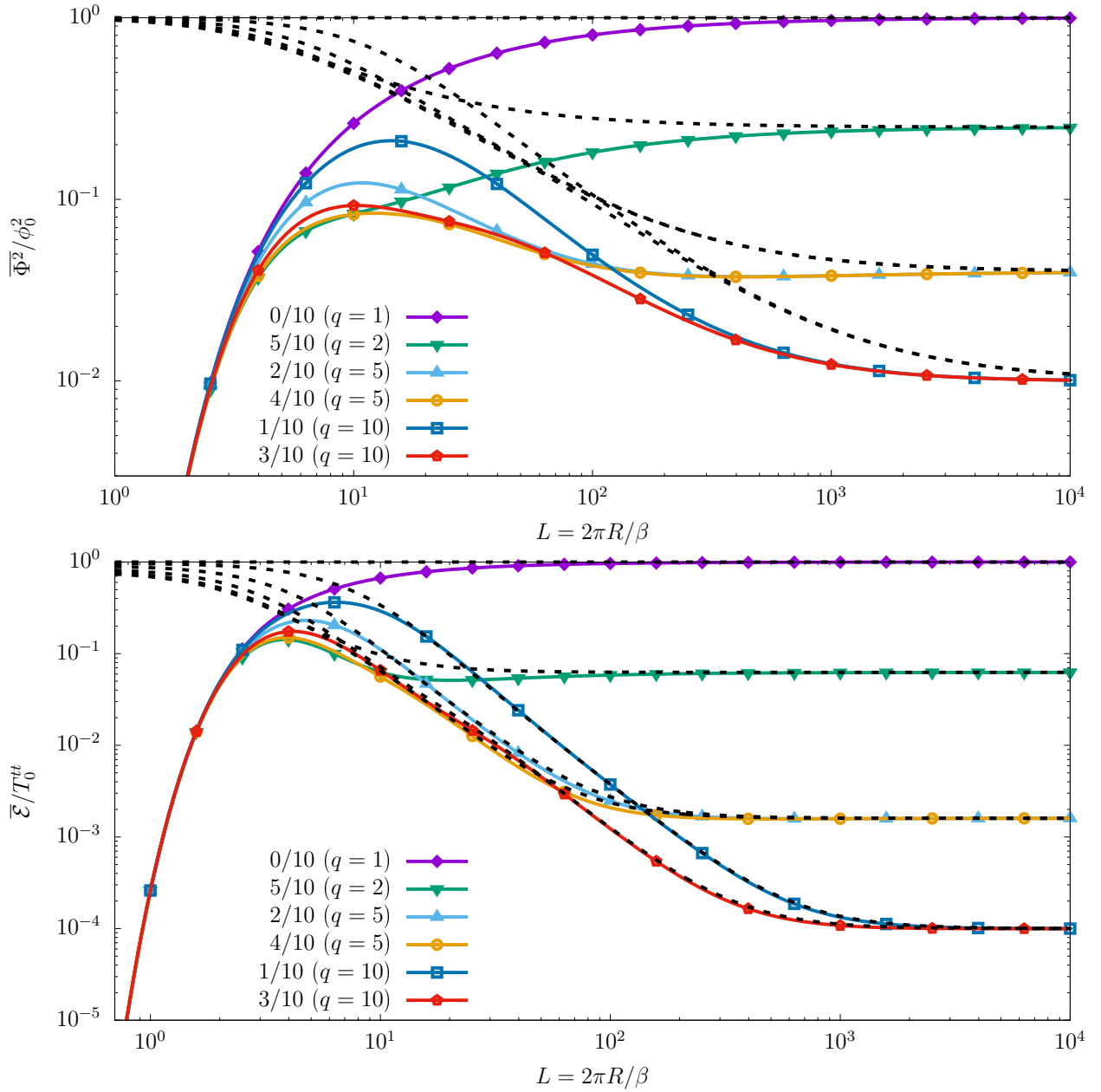
FIG. 13. Same as Fig. 8 for the case when the system is enclosed within a cylindrical boundary located at R = \beta L/2\pi , with L = 10, 100 and 1000 . The black dotted lines represent the results obtained in the unbounded case, shown in Fig. 8.
