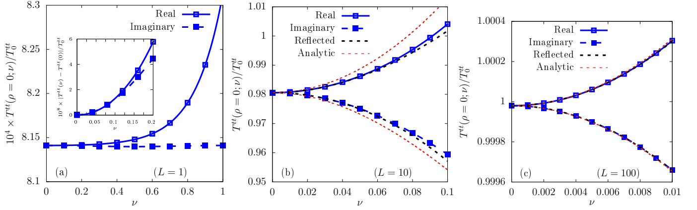
FIG. 12. Value of T^{tt}(\rho = 0; \nu) on the rotation axis with respect to T_0^{tt} = \pi^2/30\beta^4 for cylindrical systems with the dimensionless radius L = 2\pi R/\beta = 1 (a), 10 (b) and 100 (c). The rotation parameter \nu = \beta|\Omega|/2\pi (shown on the x axis) spans 0 \leq \nu \leq 1/L . The blue solid and dashed lines with squares denote results for the case of real and imaginary rotation, respectively. The black dashed lines in panels (b) and (c) are obtained by reflecting the results corresponding to real and imaginary rotation with respect to the value T^{tt}(\rho = 0; \nu = 0) obtained in the absence of rotation. The red dotted line represents the analytical expressions from the unbounded case, given in Eqs. (138b) and (143b), scaled by T^{tt}(\rho = 0; \nu = 0) .
